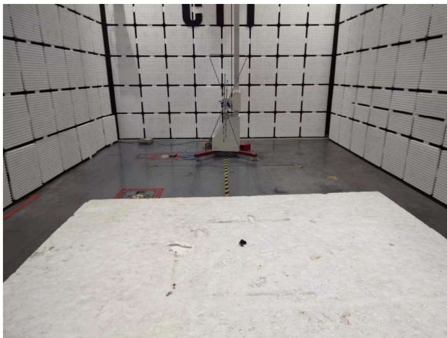
Radiated spurious emission Test Setup-1(Below 1GHz)(Ear L)
