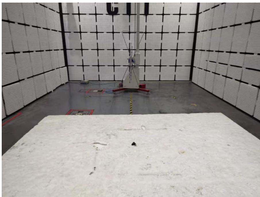
Radiated spurious emission Test Setup-1(Below 1GHz)(Ear R)
