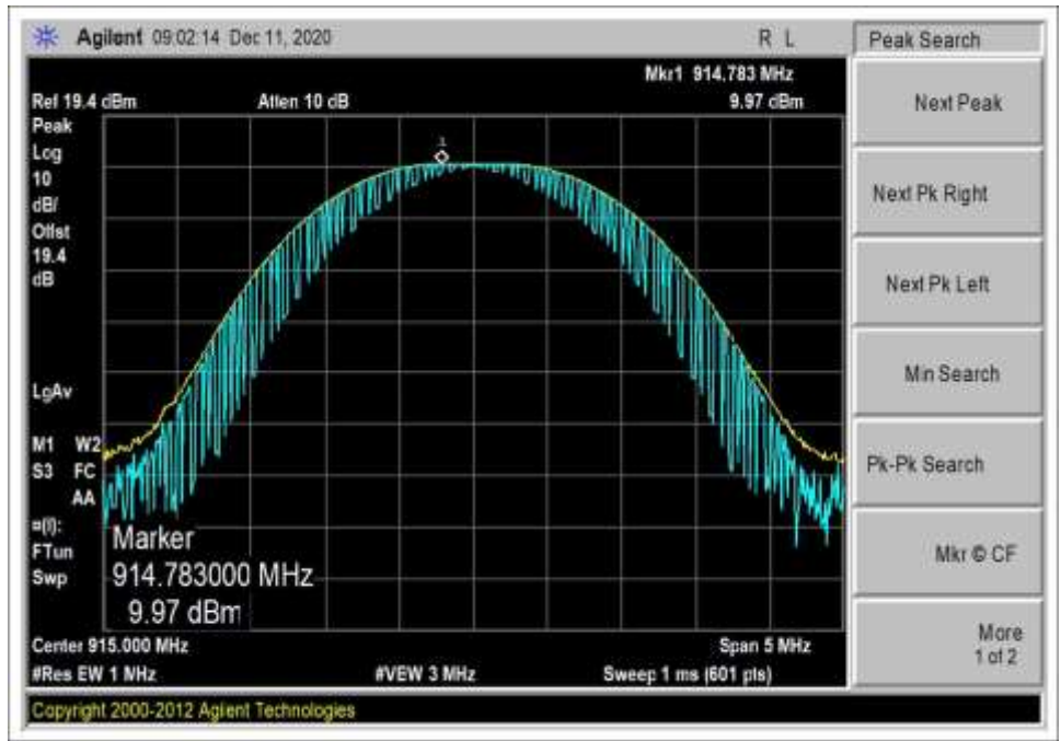
RF PWR 915M
