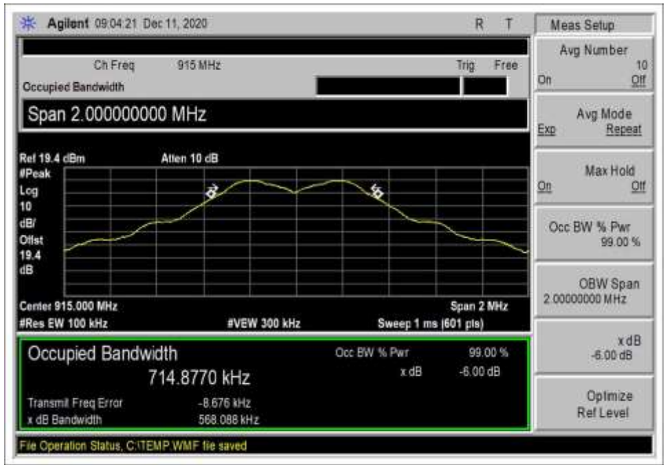
6dB BW 915M
