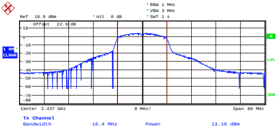
Middle channel: 2437 MHz
