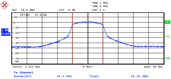
Low channel: 2412 MHz
