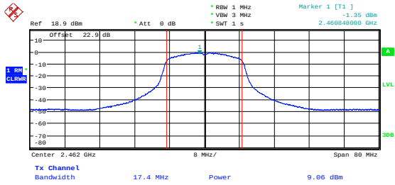
High channel: 2462 MHz
