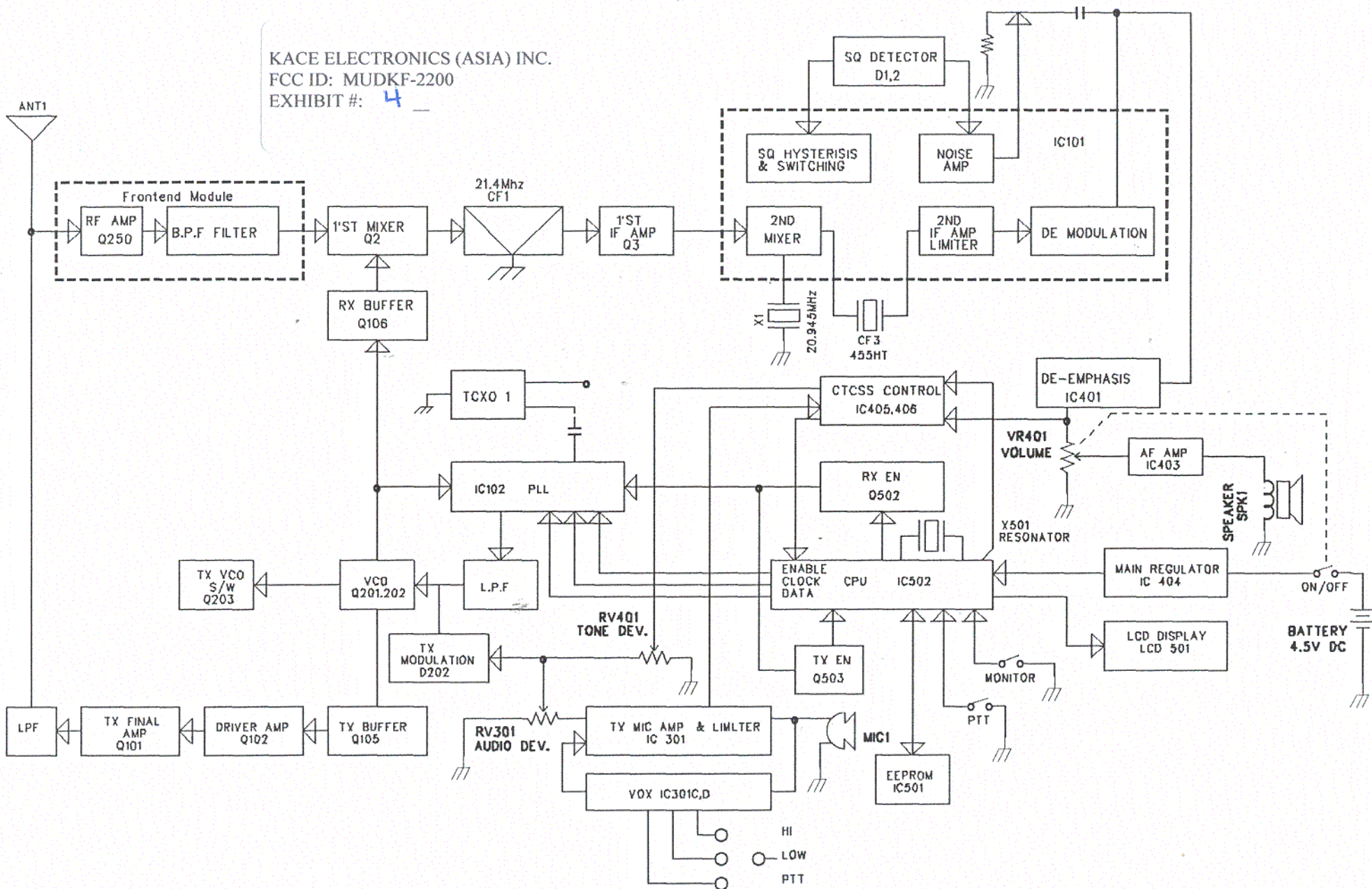
KF-2200 BLOCK DIAGRAM
