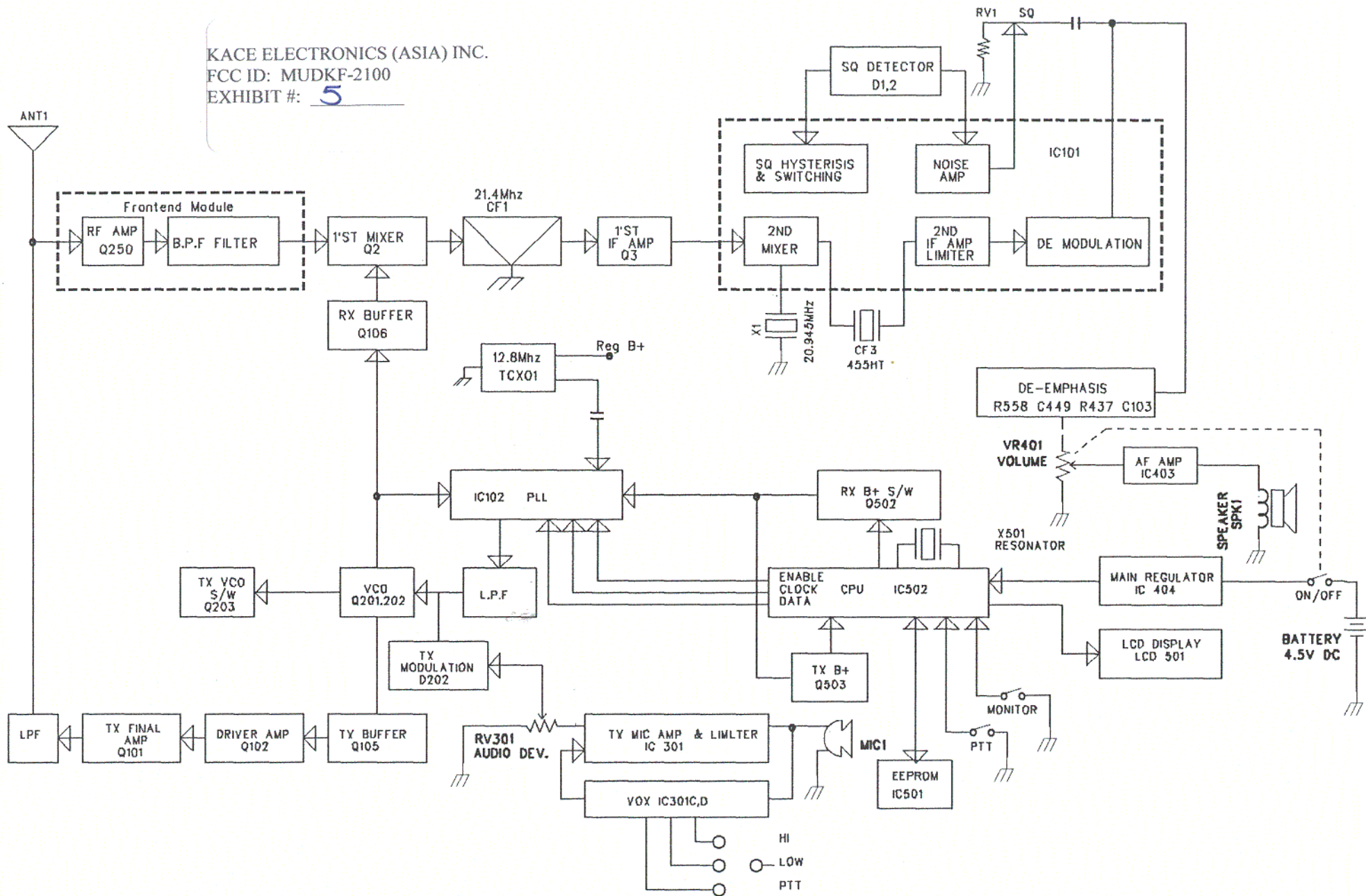
KF-2100 BLOCK DIAGRAM
