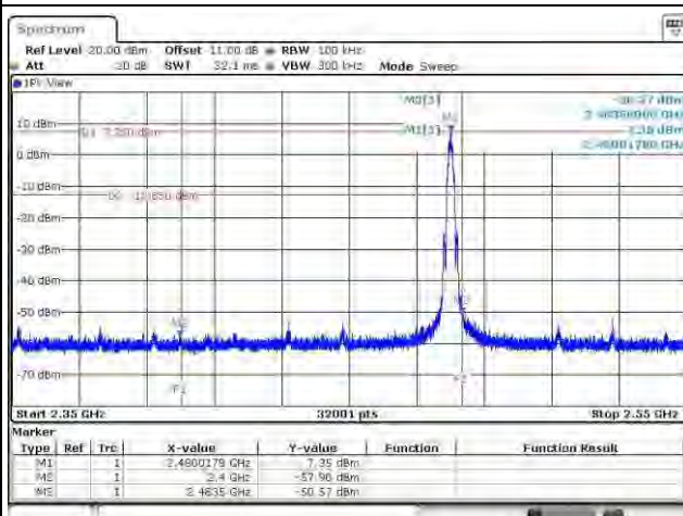
Tx 2480MHz / Reference Level
