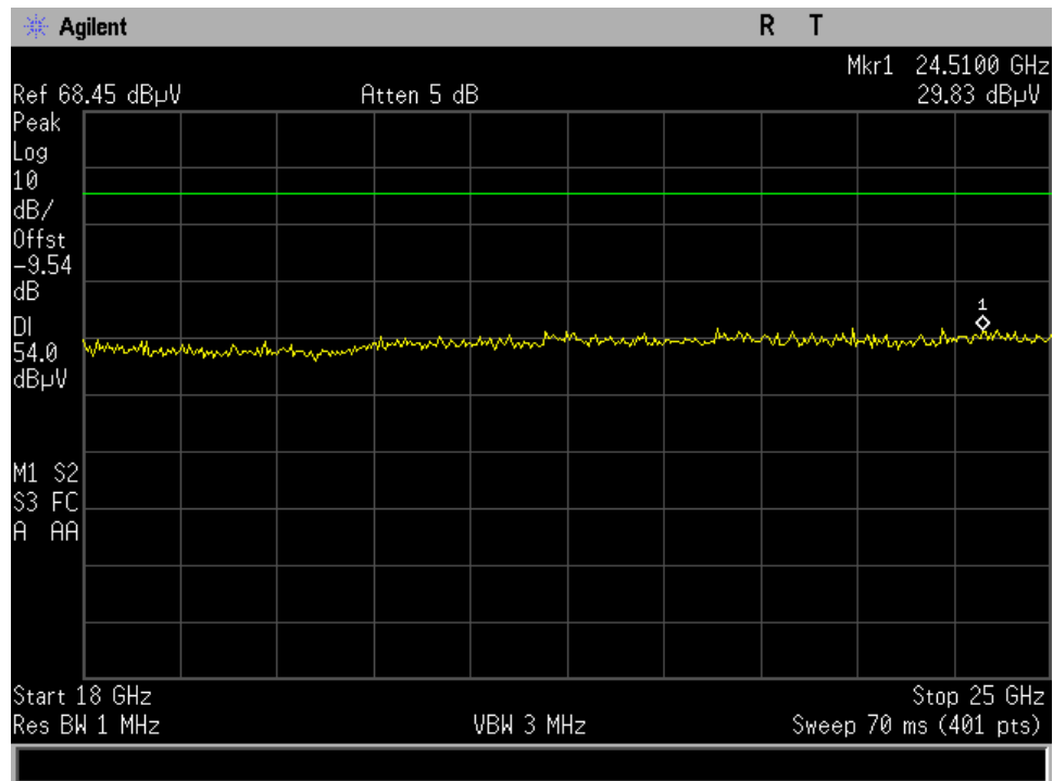
Mid Ch - 18-25 GHz - Vertical
