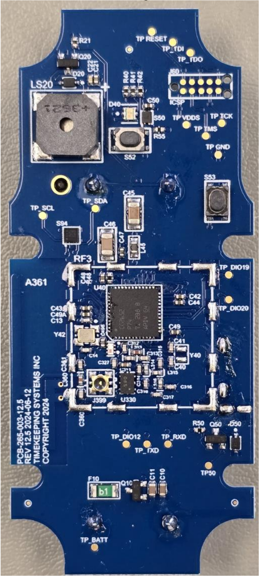
Front of Board: Cage removed
