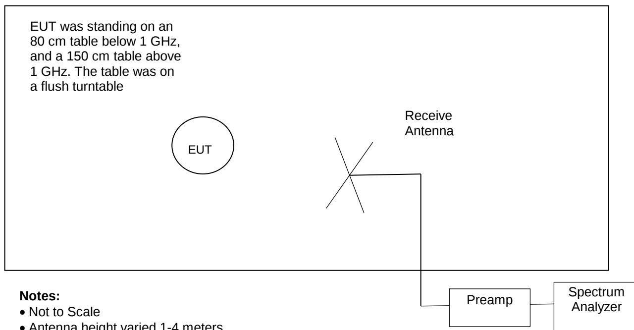
Figure 1. Drawing of Radiated Emissions Setup
