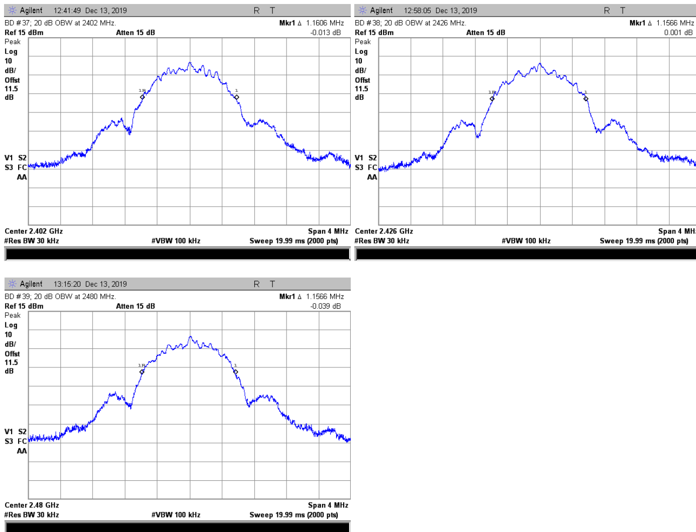
Figure 2. Occupied Bandwidth Plot
