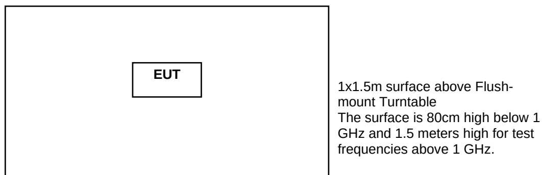
Figure 1. Drawing of Radiated Emissions Setup
