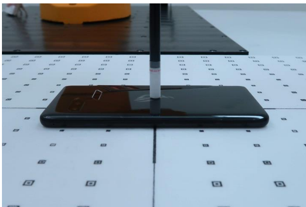
Back, Probe sensor to EUT surface distance 2mm
