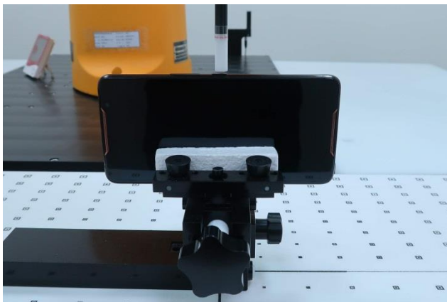
Right Side, Probe sensor to EUT surface distance
