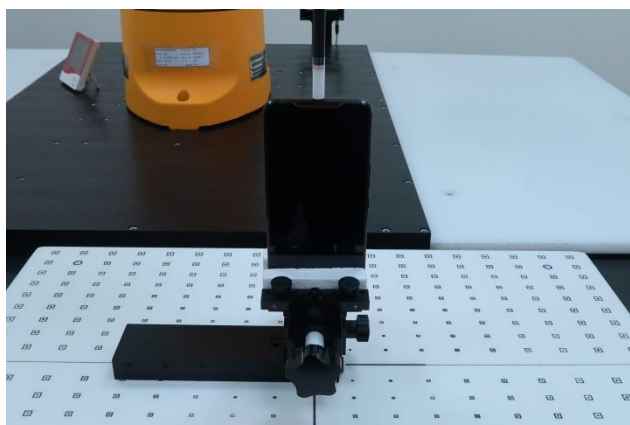
Top Side, Probe sensor to EUT surface distance 2mm
