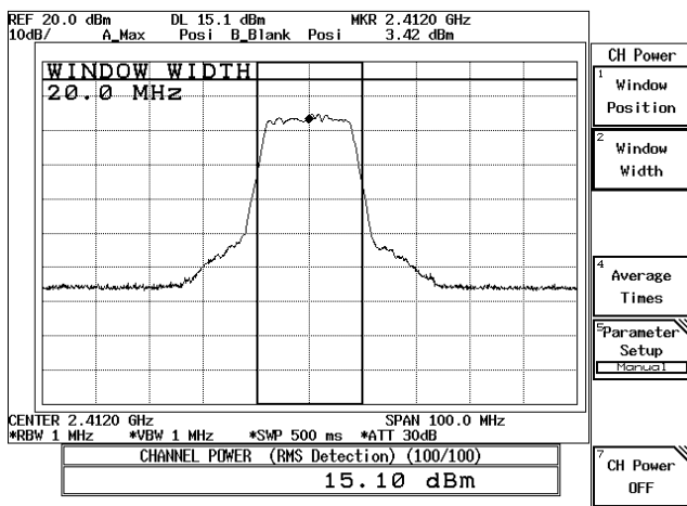
54Mbps-Ch01
