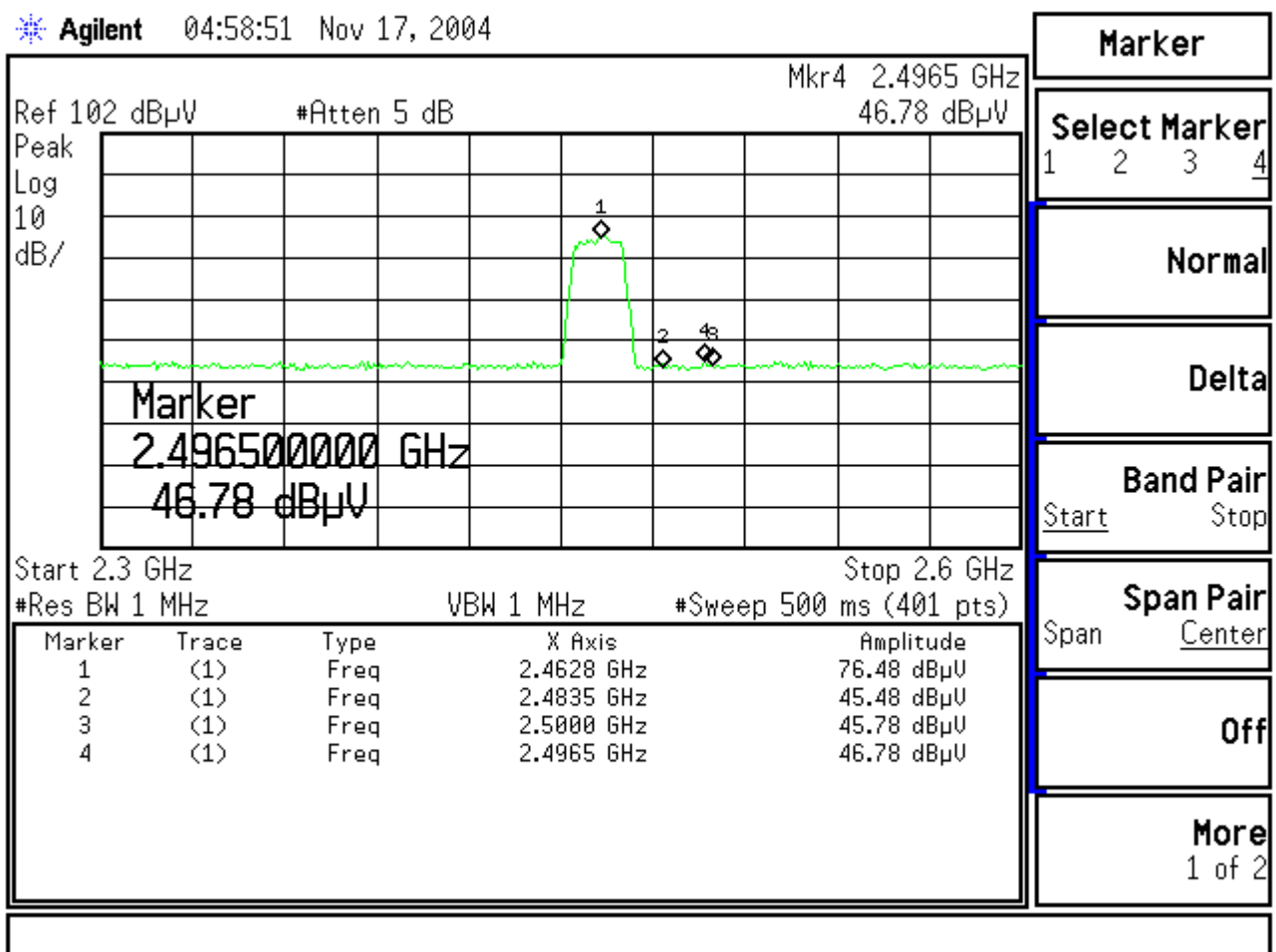
Figure Channel 11: (Vertical)
