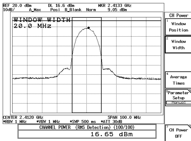
11Mbps-Ch01
