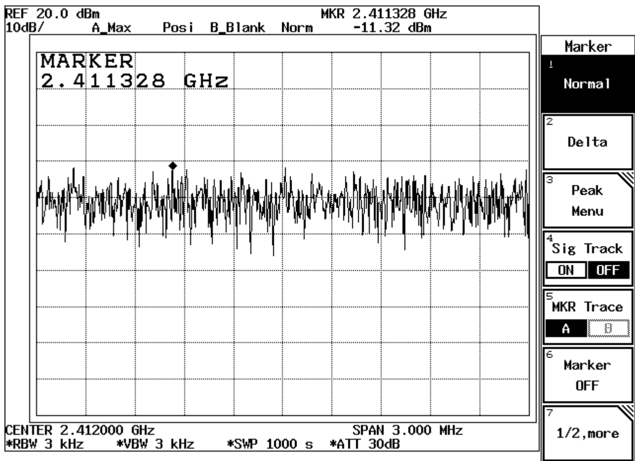
Figure Channel 1: 11Mbps
