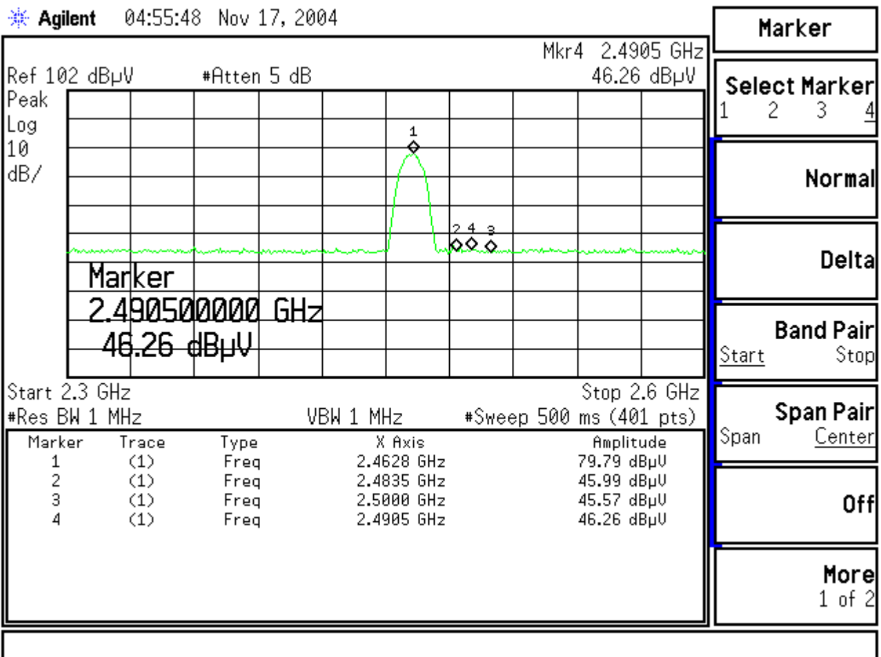
Figure Channel 11: (Vertical)
