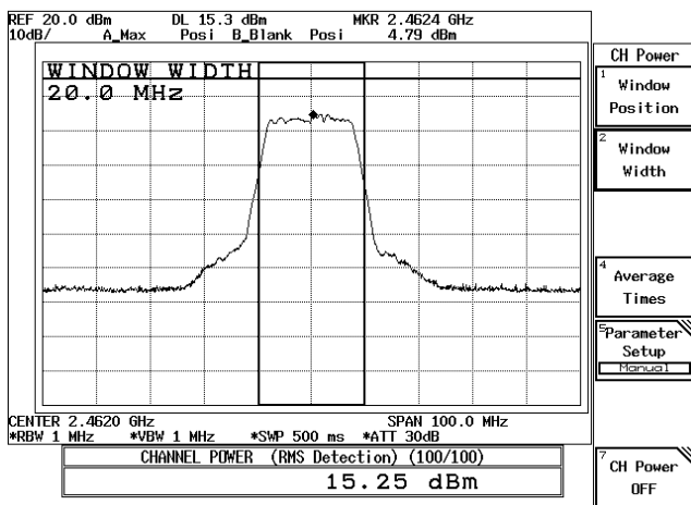
54Mbps-Ch11
