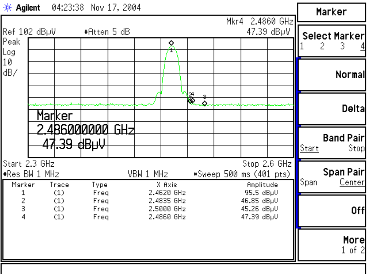
Figure Channel 11: (Horizontal)
