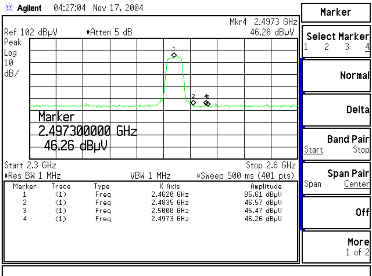
Figure Channel 11: (Horizontal)
