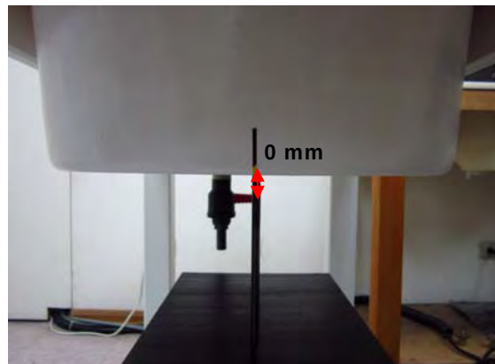
Fig.6 EUT Secondary Landscape mode to flat phantom (Test distance is 0 mm)
