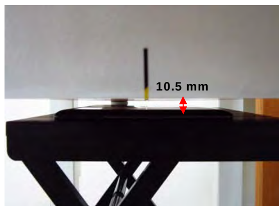
Fig.4 EUT Lap held mode to flat phantom (Test distance is 10.5 mm)
