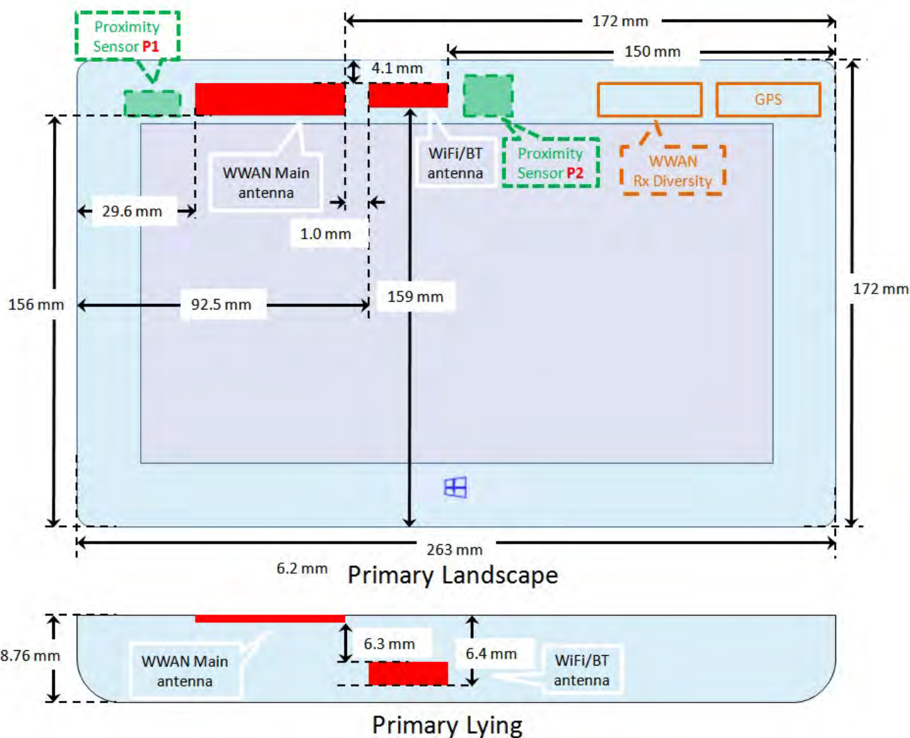
Fig.10 Antenna position of EUT
