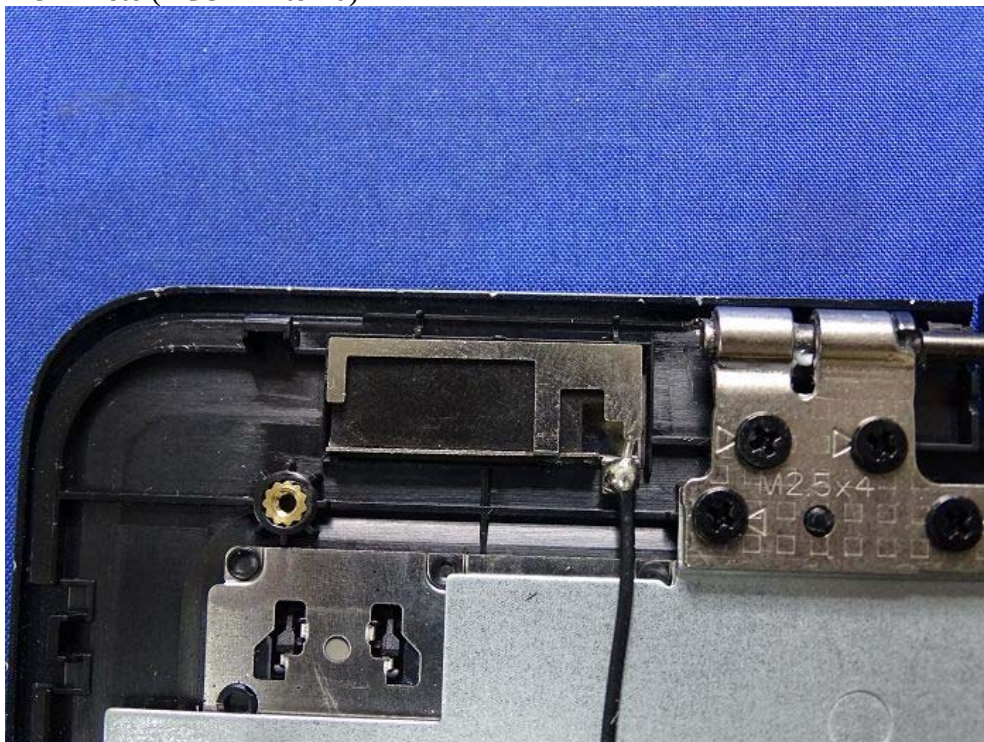
(11) EUT Photo (ACON Antenna)
