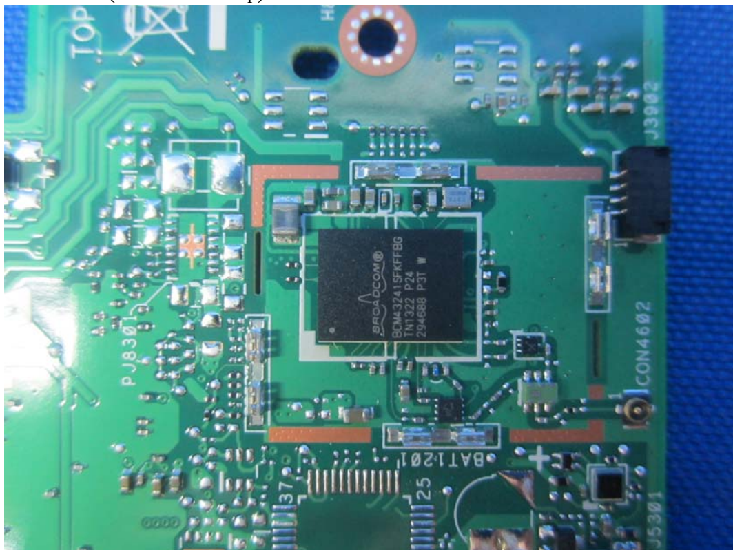
(18) EUT Photo (BT+WLAN Chip)
