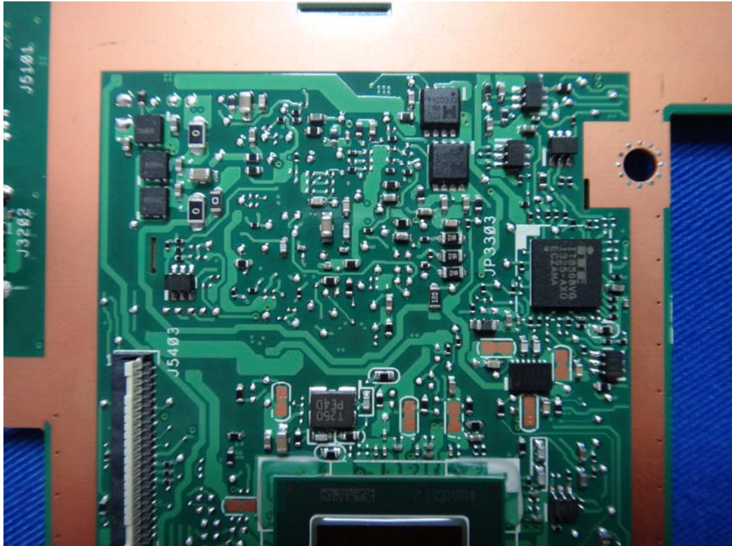
(22) EUT Photo (Antenna)
