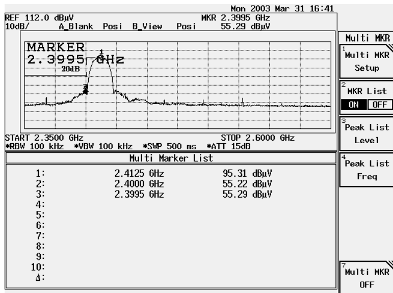
Figure Channel 1: (Vertical)
