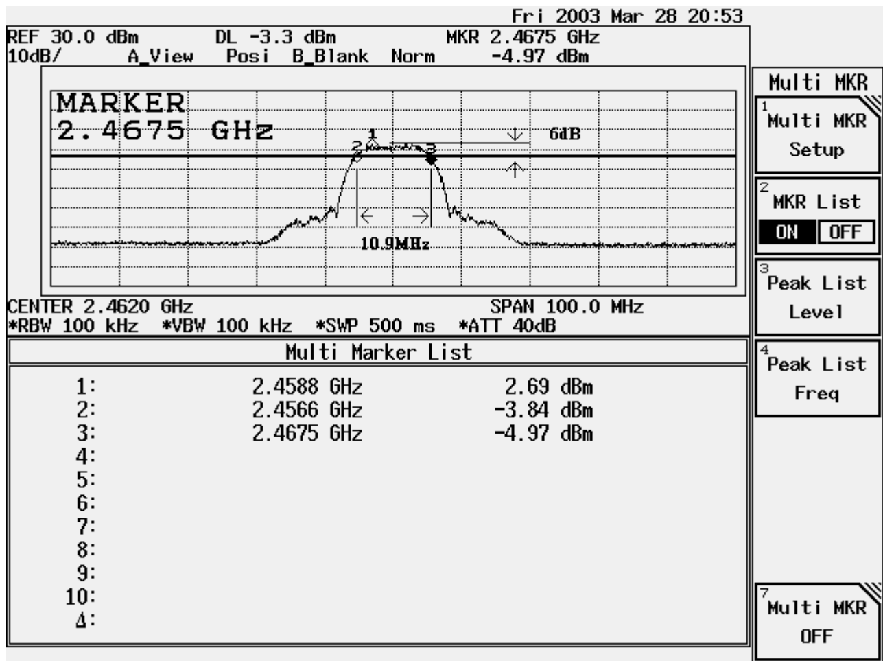
Figure Channel 11: 11Mbps
