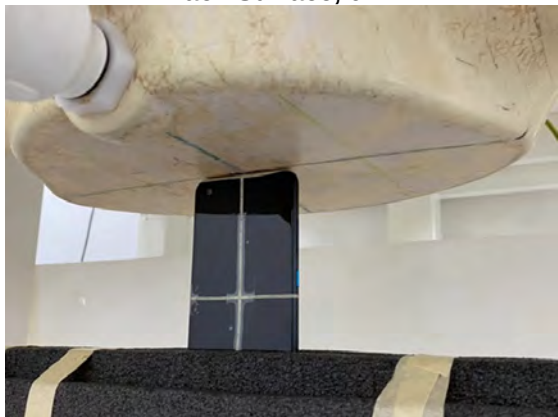
Photograph 29. Product specific 10-g SAR, Top Edge, 0mm
