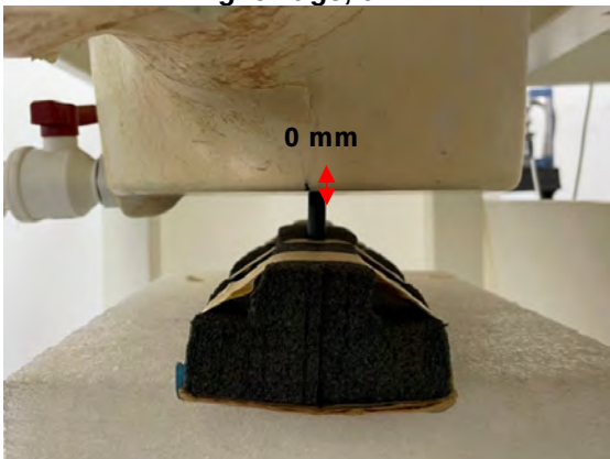
Photograph 36. Product specific 10-g SAR, Left Edge, 0mm
