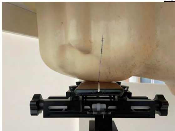
Photograph 1. Head, Right Touch, 0mm
