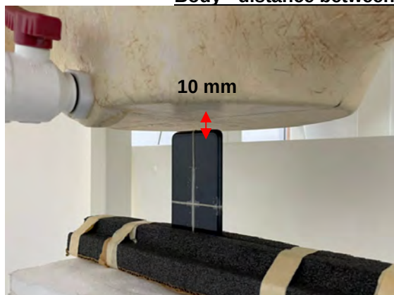
Photograph 19. Hotspot, Bottom Edge, 10mm
