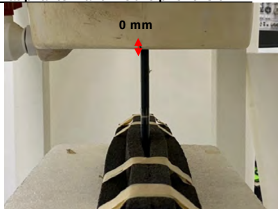
Photograph 32. Product specific 10-g SAR, Bottom Edge, 0mm
