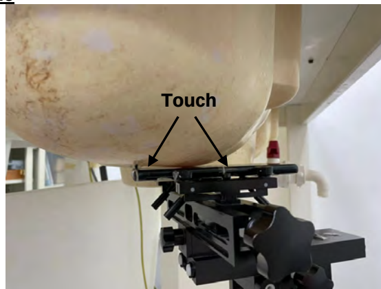
Photograph 2. Head, Right Touch, 0mm
