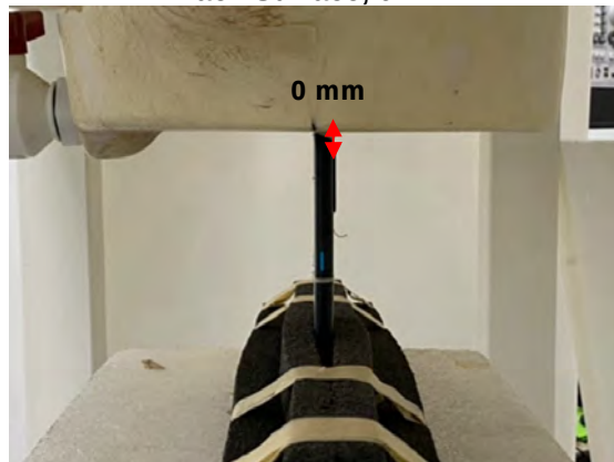
Photograph 30. Product specific 10-g SAR, Top Edge, 0mm
