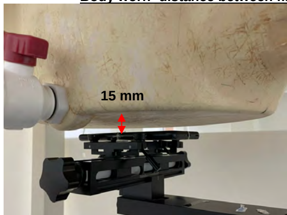
Photograph 9. Body-worn, Front Surface, 15mm
