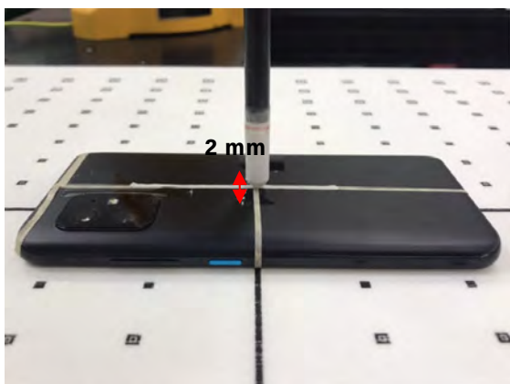
Photograph 39. PD, Back Surface, 2mm
