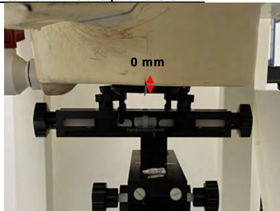
Photograph 26. Product specific 10-g SAR, Front Surface, 0mm
