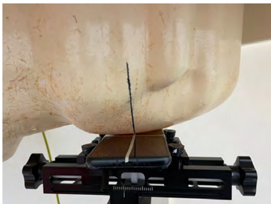
Photograph 5. Head, Left Touch, 0mm
