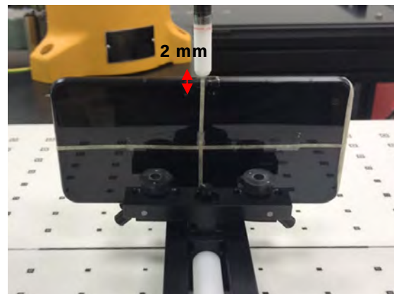
Photograph 41. PD, Left Edge, 2mm
