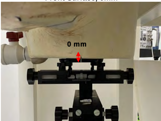
Photograph 28. Product specific 10-g SAR, Back Surface, 0mm
