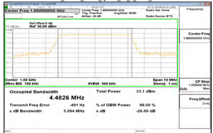
DFT-s-OFDM_Band2_5MHz_QPSK_25_0_Main_MidCH376000
