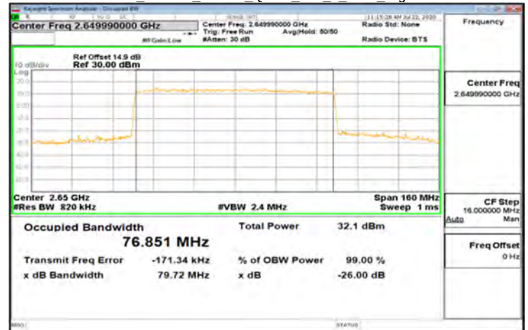
DFT-s-OFDM_Band41_80MHz_QPSK_216_0_Main_HighCH529998
