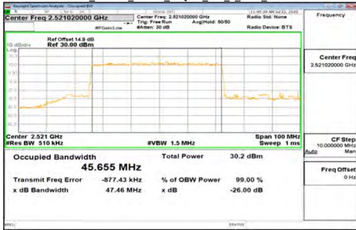
DFT-s-OFDM Band41_50MHz_16QAM_128_0_Main_LowCH504204
