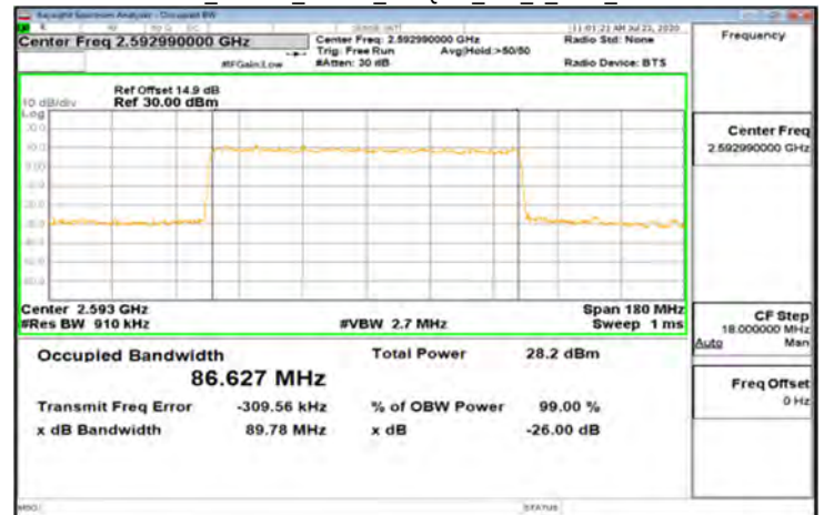
DFT-s-OFDM_Band41_90MHz_256QAM_243_0_Main_MidCH518598
