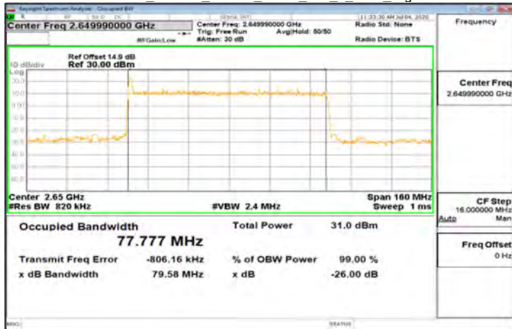
DFT-s-OFDM Pi/2_Band41_80MHz_BPSK_216_0_Main_HighCH529998
