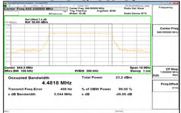
DFT-s-OFDM_Band5_5MHz_QPSK_25_0_Main_HighCH169300
