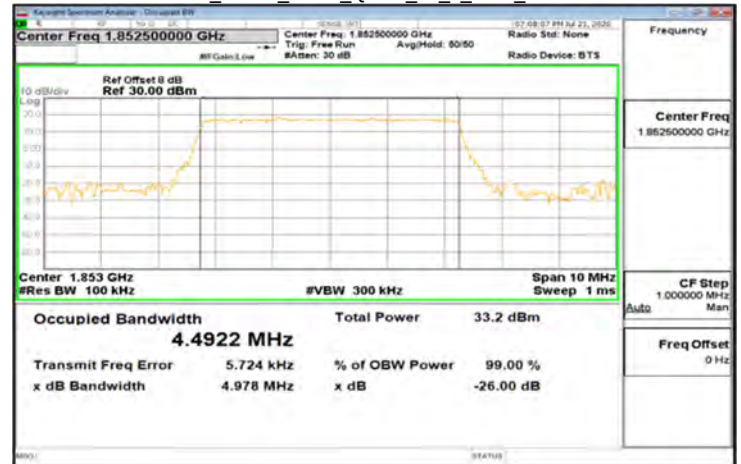
DFT-s-OFDM_Band2_5MHz_QPSK_25_0_Main_LowCH370500
