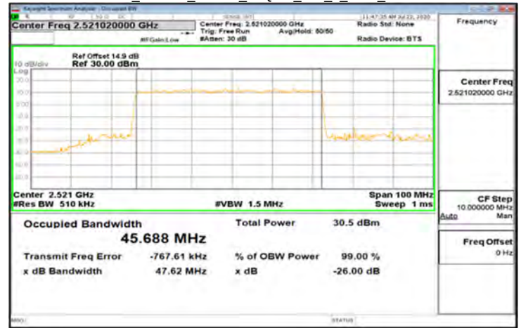
DFT-s-OFDM Band41_50MHz_64QAM_128_0_Main_LowCH504204
