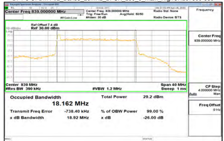
DFT-s-OFDM Pi/2_Band5_20MHz_BPSK_100_0_Main_HighCH167800-839
