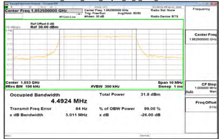
DFT-s-OFDM_Band2_5MHz_64QAM_25_0_Main_LowCH370500
