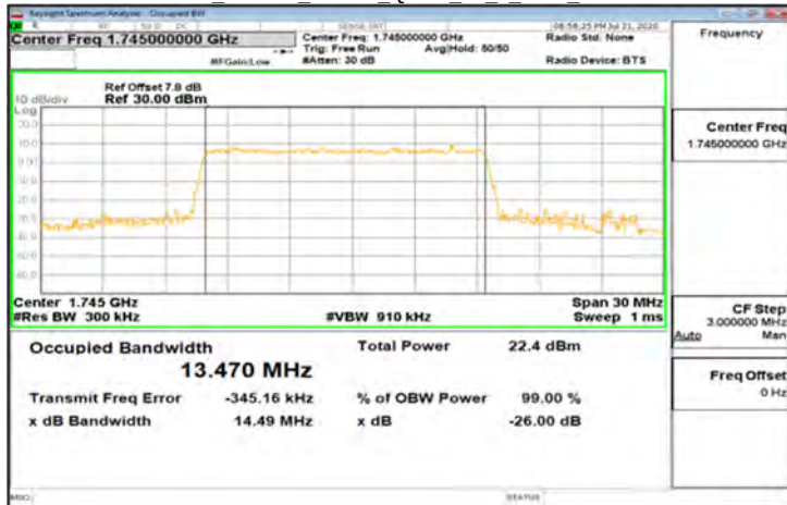
DFT-s-OFDM_Band66_15MHz_QPSK_75_0_Main_MidCH349000
