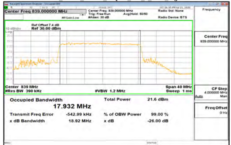
DFT-s-OFDM_Band5_20MHz_16QAM_100_0_Main_HighCH167800
