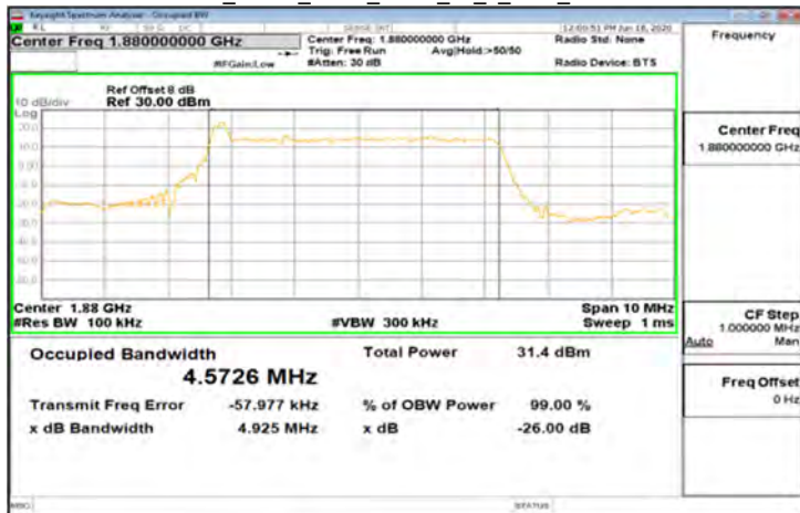
DFT-s-OFDM Pi/2_Band2_5MHz_BPSK_25_0_Main_MidCH376000-1880
