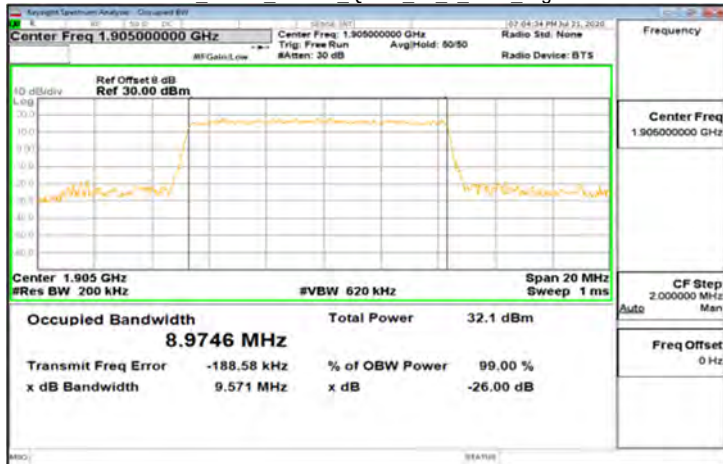
DFT-s-OFDM_Band2_10MHz_QPSK_50_0_Main_HighCH381000
