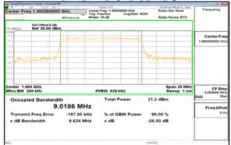
DFT-s-OFDM_Band2_10MHz_16QAM_50_0_Main_HighCH381000
