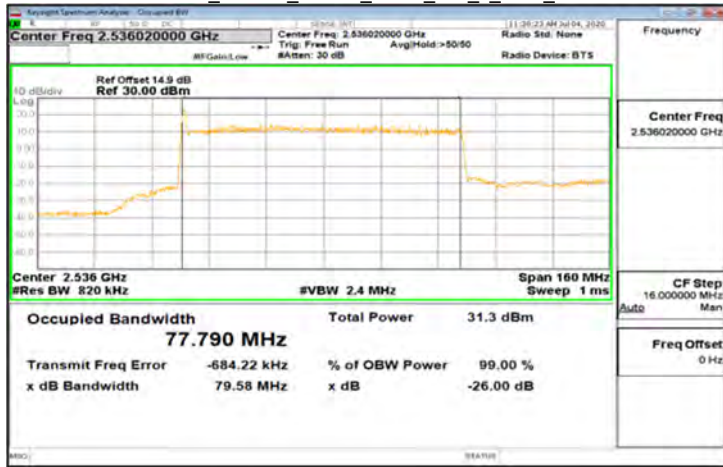
DFT-s-OFDM Pi/2_Band41_80MHz_BPSK_216_0_Main_LowCH507204
