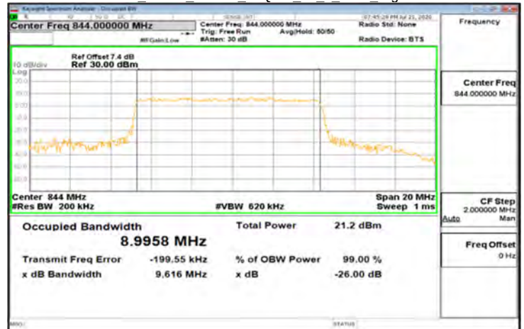
DFT-s-OFDM_Band5_10MHz_16QAM_50_0_Main_HighCH168800
