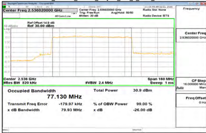
DFT-s-OFDM_Band41_80MHz_16QAM_216_0_Main_LowCH507204
