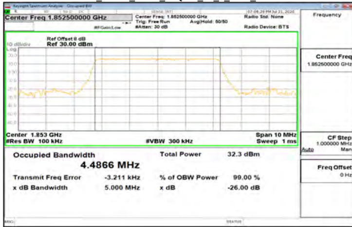
DFT-s-OFDM_Band2_5MHz_16QAM_25_0_Main_LowCH370500
