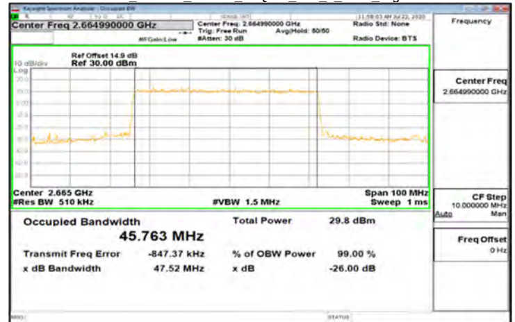
DFT-s-OFDM Band41_50MHz_64QAM_128_0_Main_HighCH532998
