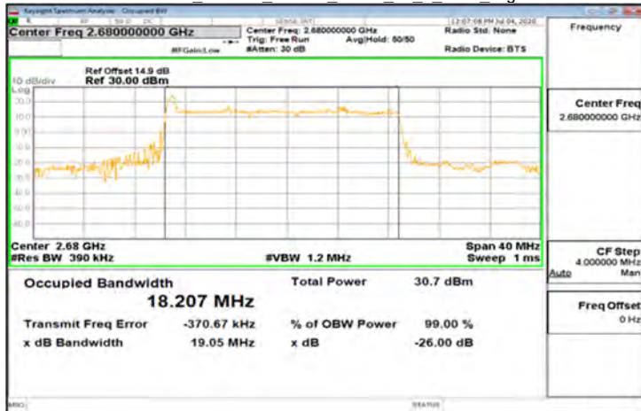
DFT-s-OFDM Pi/2_Band41_20MHz_BPSK_50_0_Main_HighCH41490
