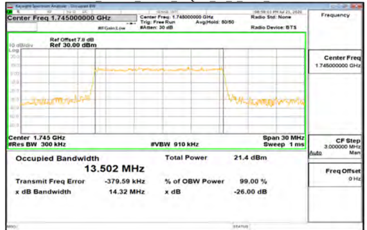
DFT-s-OFDM_Band66_15MHz_16QAM_75_0_Main_MidCH349000
