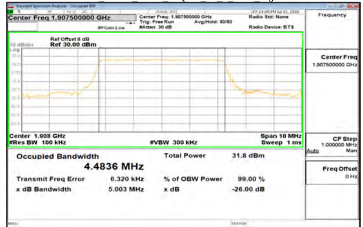
DFT-s-OFDM_Band2_5MHz_64QAM_25_0_Main_HighCH381500
