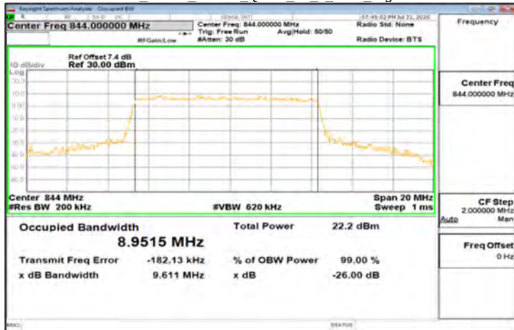
DFT-s-OFDM_Band5_10MHz_QPSK_50_0_Main_HighCH168800
