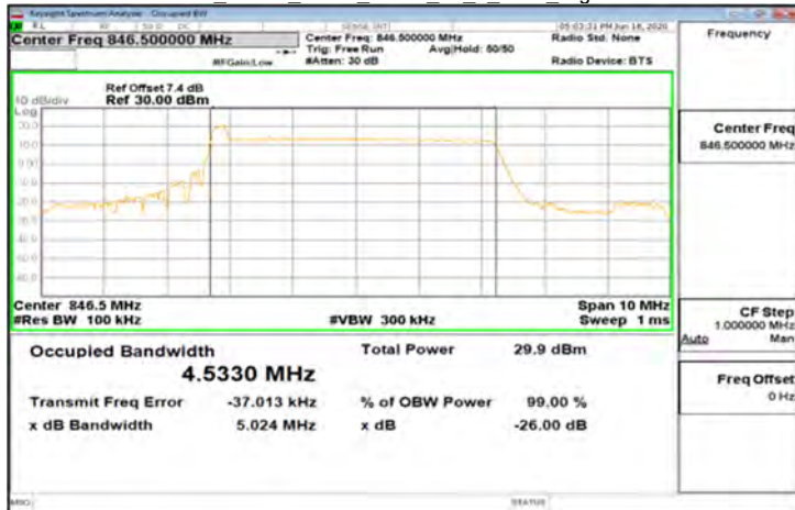
DFT-s-OFDM Pi/2_Band5_5MHz_BPSK_25_0_Main_HighCH169300-846.5
