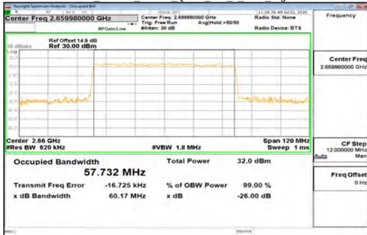
DFT-s-OFDM_Band41_60MHz_QPSK_162_0_Main_HighCH534996
