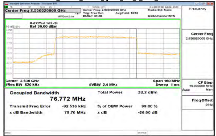
DFT-s-OFDM_Band41_80MHz_QPSK_216_0_Main_LowCH507204
