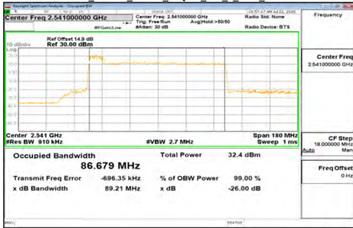
DFT-s-OFDM_Band41_90MHz_64QAM_243_0_Main_LowCH508200
