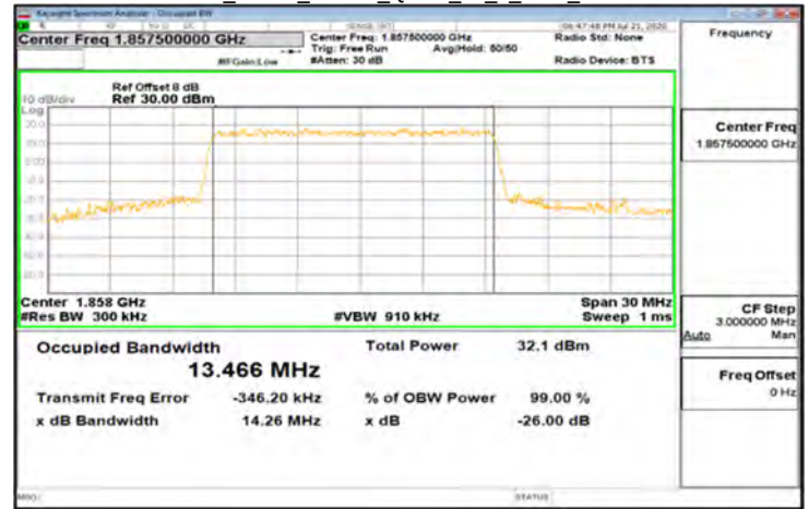
DFT-s-OFDM_Band2_15MHz_QPSK_75_0_Main_LowCH371500
