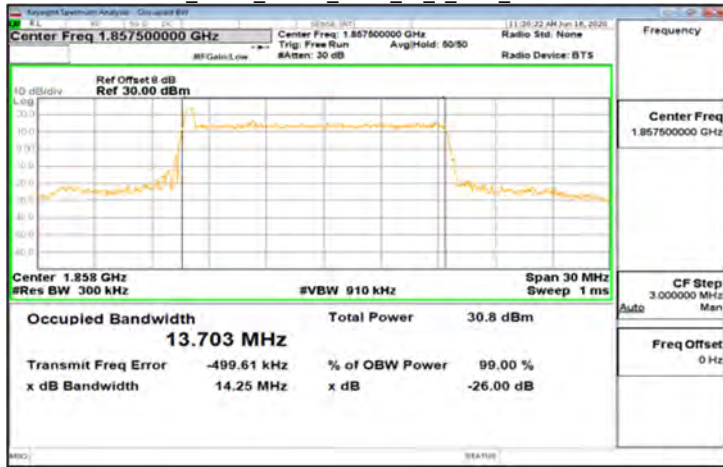
DFT-s-OFDM Pi/2_Band2_15MHz_BPSK_75_0_Main_LowCH371500-1857.5
