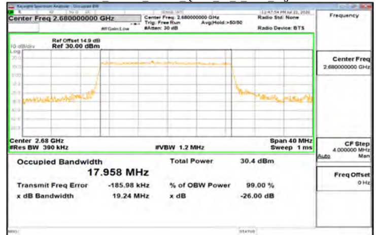
DFT-s-OFDM Band41_20MHz_QPSK_50_0_Main_HighCH41490
