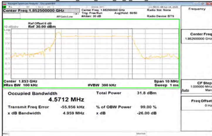
DFT-s-OFDM Pi/2_Band2_5MHz_BPSK_25_0_Main_LowCH370500-1852.5
