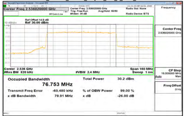
DFT-s-OFDM_Band41_80MHz_64QAM_216_0_Main_LowCH507204
