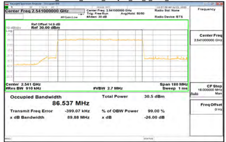
DFT-s-OFDM_Band41_90MHz_256QAM_243_0_Main_LowCH508200
