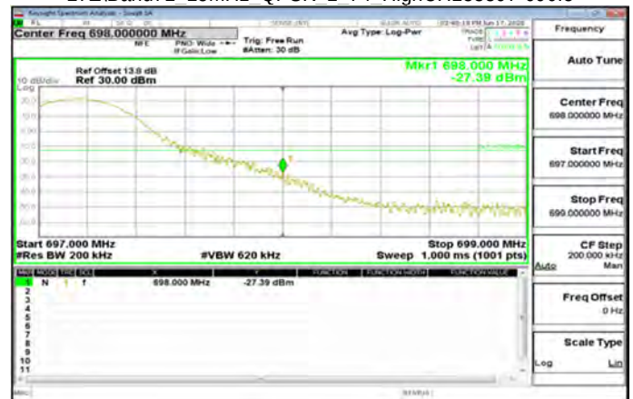
LTE\Band71_15MHz_QPSK_1_74_HighCH133397-690.5
