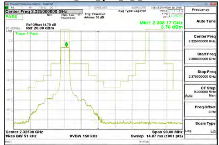
Band30 5MHz_QPSK 25 0 CH27735
