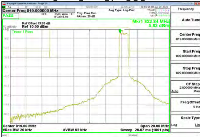
Band26 Part90s 1.4MHz QPSK 6 0 CH26783
