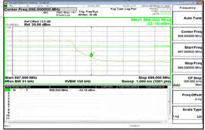
LTE\Band71_5MHz_QPSK_25_0_HighCH133447-695.5
