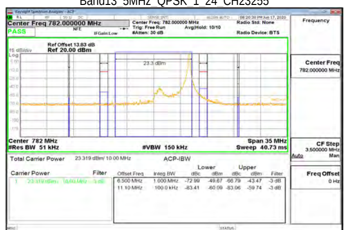
Band13 5MHz QPSK 1 24 CH23255
