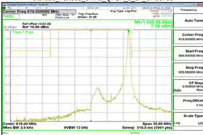
Band26_Part90s_5MHz_QPSK_1_24_CH26765
