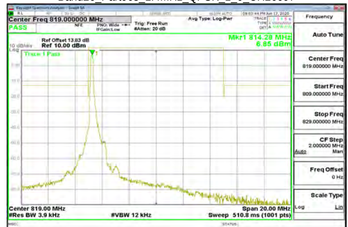
Band26 Part90s_1.4MHz_QPSK_1_0_CH26697
