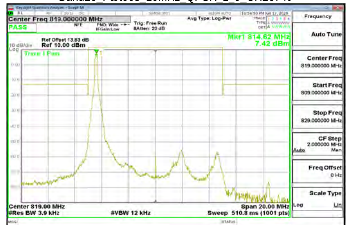
Band26_Part90s_10MHz_QPSK_1_0_CH26740
