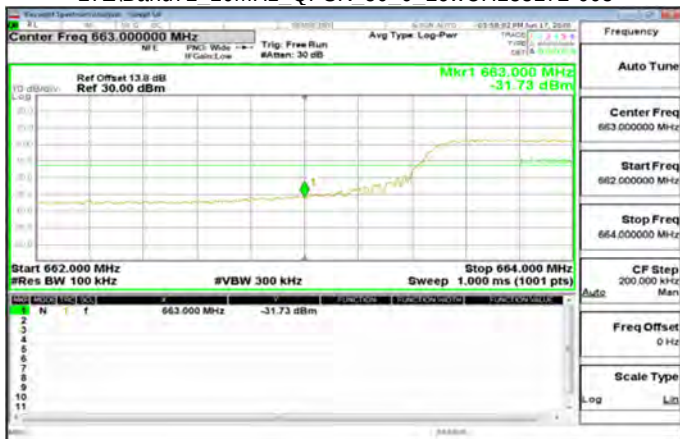
LTE\Band71_10MHz_QPSK_50_0_LowCH133172-668
