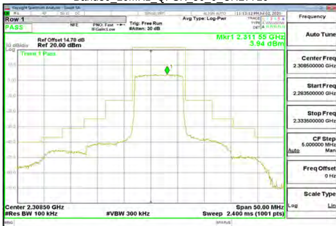
Band30_10MHz_QPSK_50_0_CH27710
