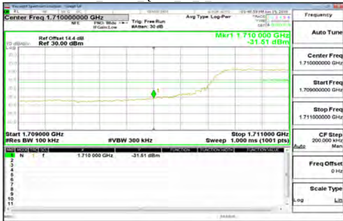
LTE\Band66_10MHz_QPSK_50_0_LowCH132022-1715
