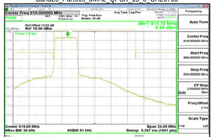
Band26 Part90s 3MHz QPSK 15 0 CH26705
