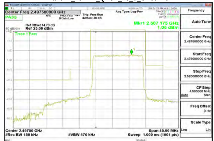
Band41_15MHz_QPSK_75_0_CH39725
