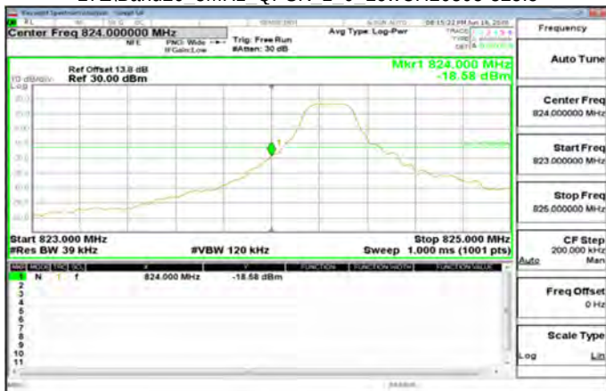
LTE\Band26_3MHz_QPSK_1_0_LowCH26805-825.5
