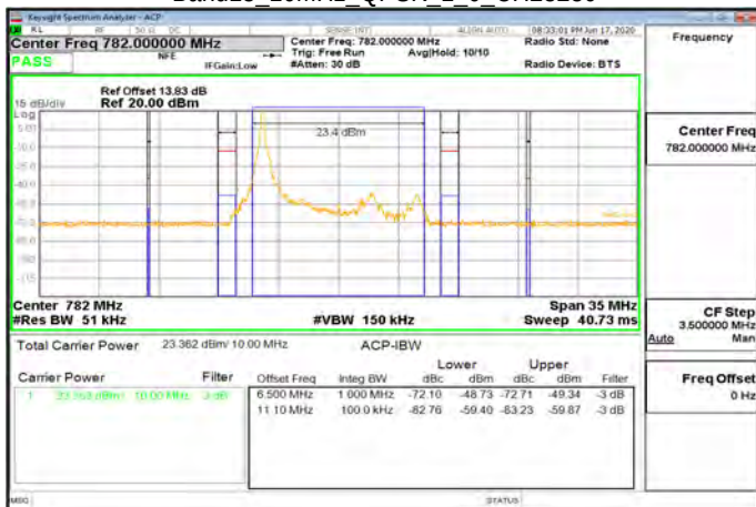
Band13 10MHz_QPSK_1_0_CH23230
