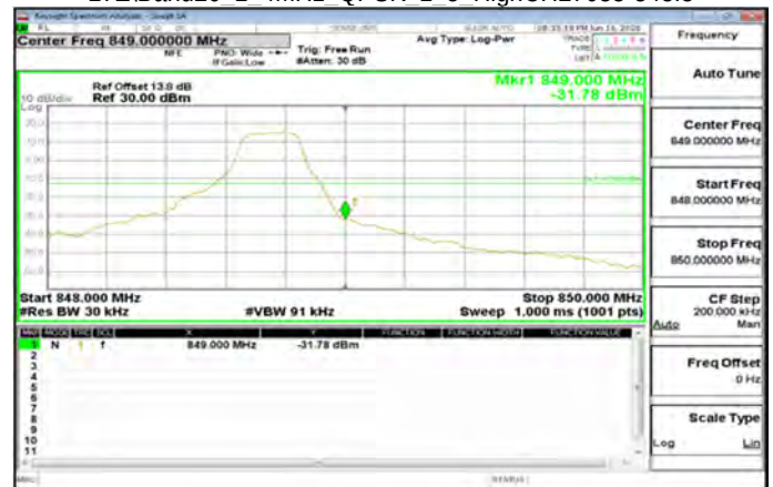
LTE\Band26_1_4MHz_QPSK_1_5_HighCH27033-848.3
