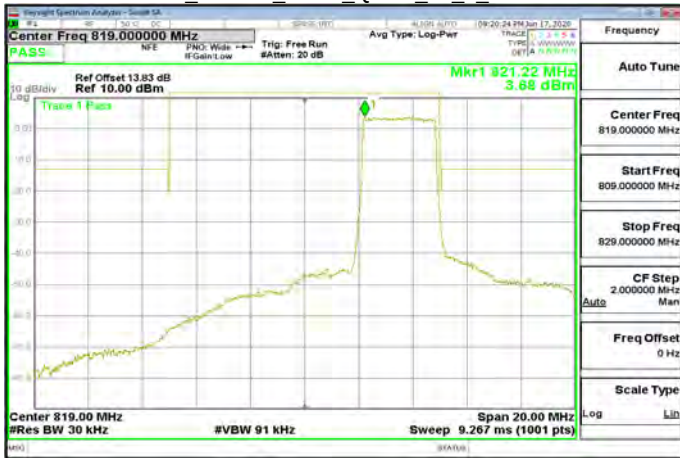
Band26_Part90s_5MHz_QPSK_1_0_CH26715
