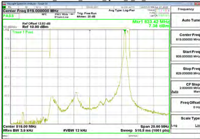
Band26 Part90s 10MHz_QPSK 50 0 CH26740
