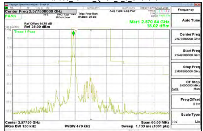
Band38 15MHz_QPSK 1 0 CH37825
