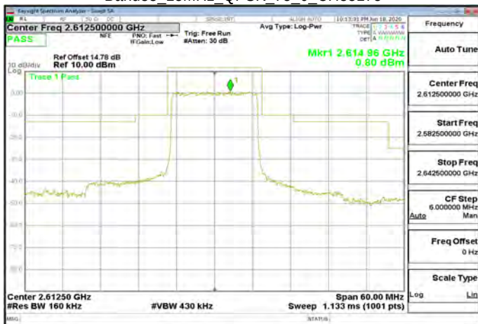
Band38 15MHz QPSK 75 0 CH38175
