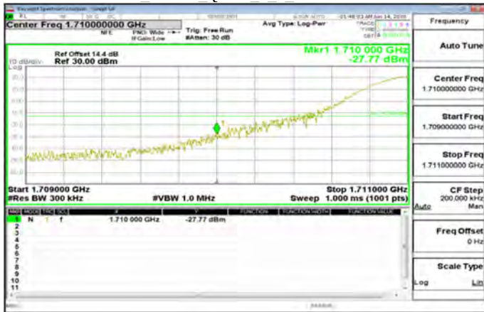
LTE\Band66_20MHz_QPSK_1_0_LowCH132072-1720
