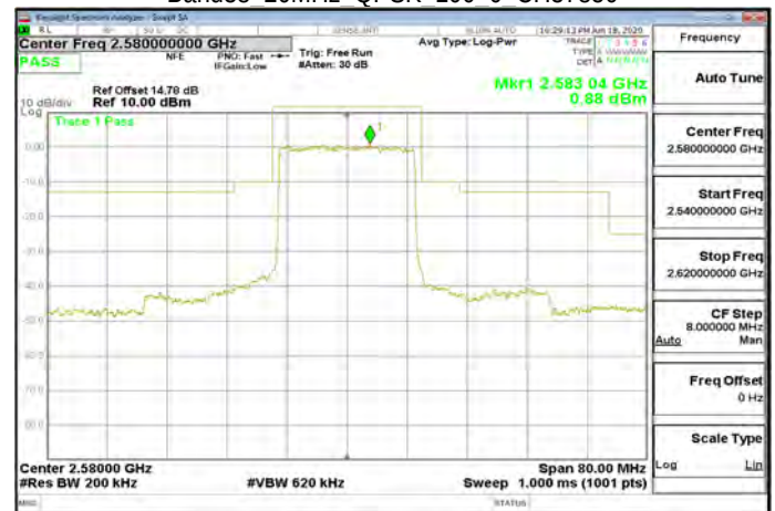
Band38 20MHz QPSK 100 0 CH37850
