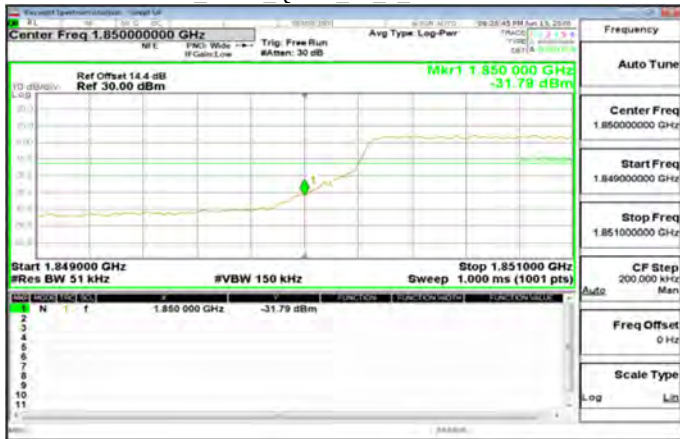
LTE\Band25_5MHz_QPSK_25_0_LowCH26065-1852.5
