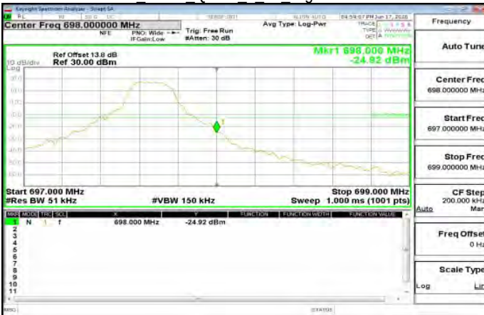
LTE\Band71_5MHz_QPSK_1_24_HighCH133447-695.5
