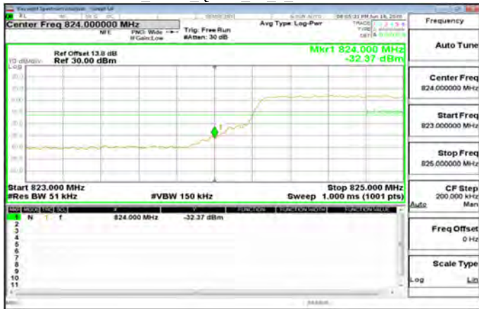
LTE\Band26_5MHz_QPSK_25_0_LowCH26815-826.5
