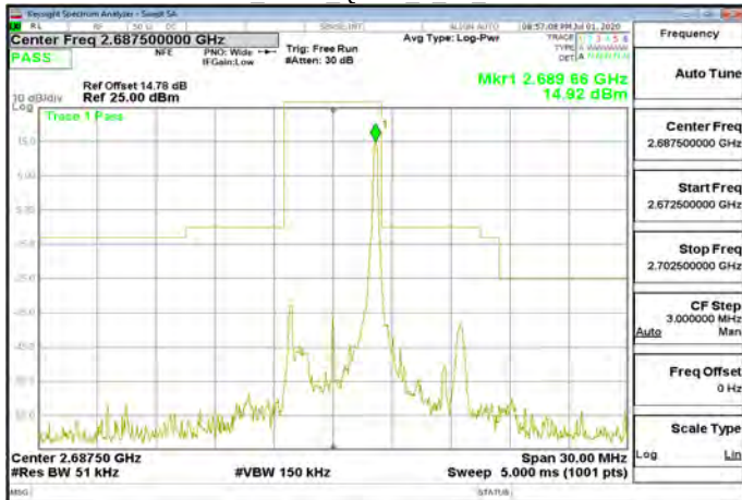
Band41 5MHz_QPSK 1 24 CH41565
