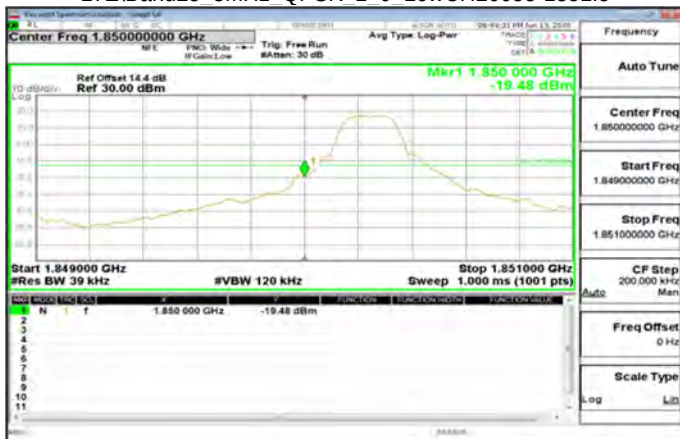
LTE\Band25_3MHz_QPSK_1_0_LowCH26055-1851.5
