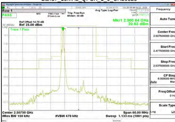
Band7 15MHz QPSK 1 0 CH20825
