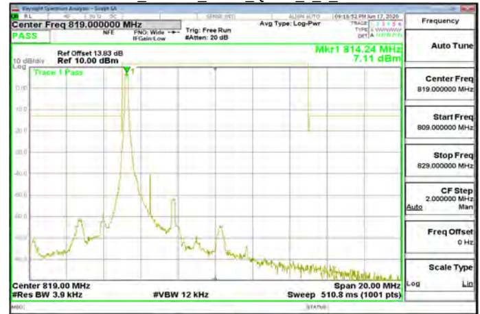
Band26 Part90s 3MHz QPSK 1 14 CH26775
