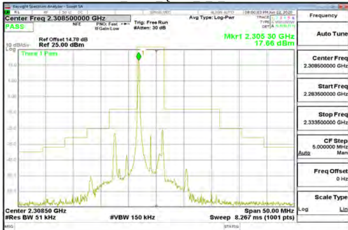
Band30 5MHz_QPSK 1 0 CH27685
