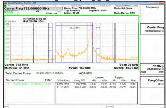
Band13 10MHz_QPSK_50_0_CH23230
