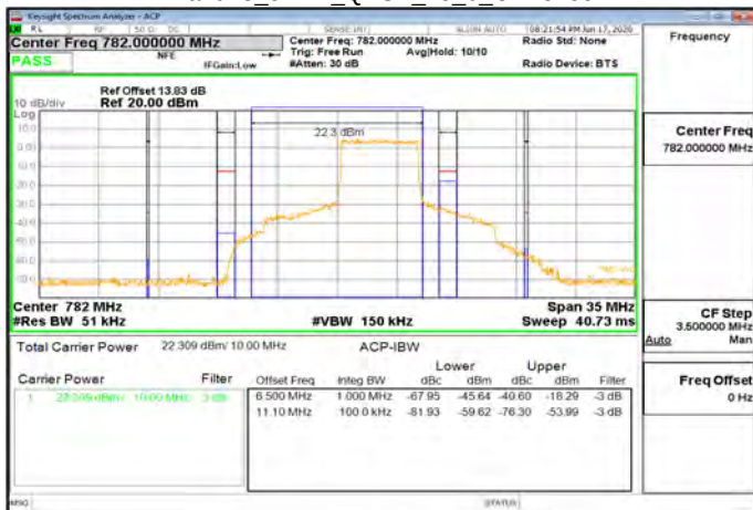
Band13 10MHz_QPSK_1_0_CH23230
