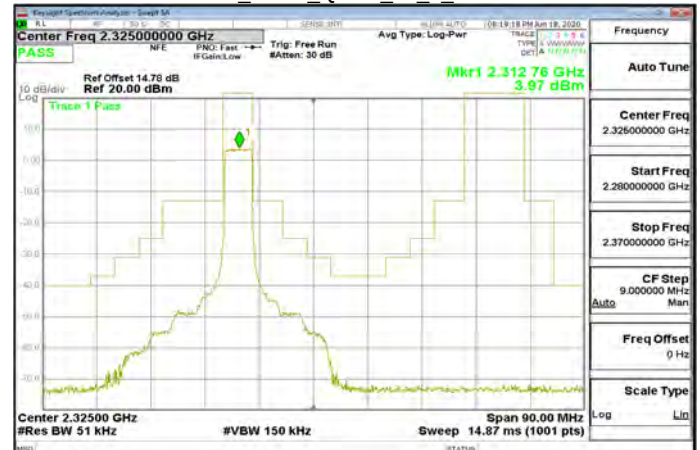
Band30 5MHz_QPSK 25 0 CH27735
