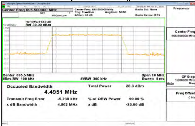
Band71 5MHz 64QAM 25 0 Main HighCH133447-695.5
