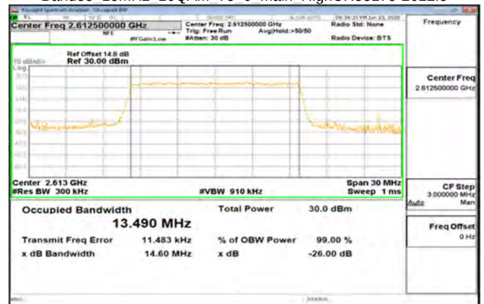
Band38 15MHz 16QAM 75 0 Main HighCH38175-2612.5
