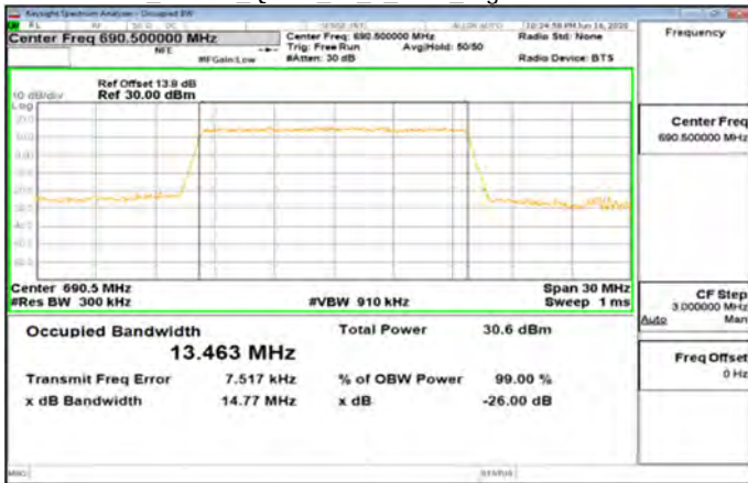
Band71 15MHz QPSK 75 0 Main HighCH133397-690.5
