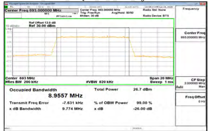
Band71 10MHz 256QAM 50 0 Main HighCH133422-693
