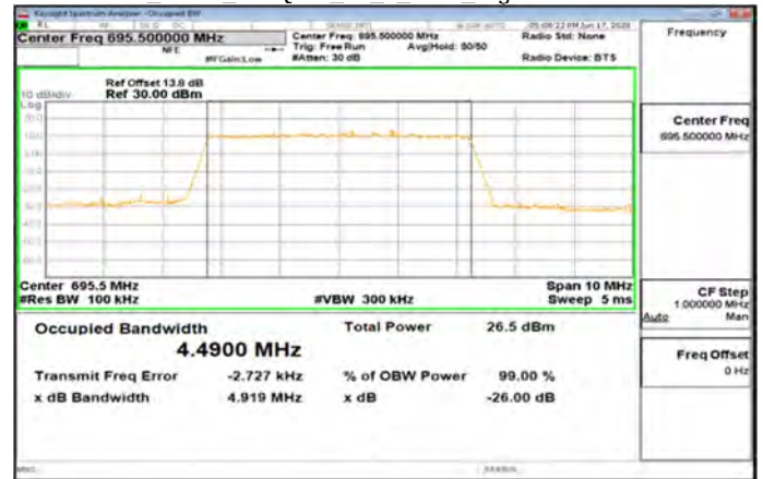
Band71 5MHz 256QAM 25 0 Main HighCH133447-695.5
