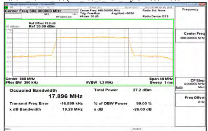
Band71 20MHz 256QAM 100 0 Main HighCH133372-688
