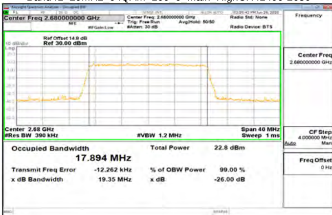
Band41 20MHz 64QAM 100 0 Main HighCH41490-2680
