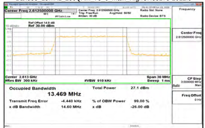
Band38 15MHz 256QAM 75 0 Main HighCH38175-2612.5
