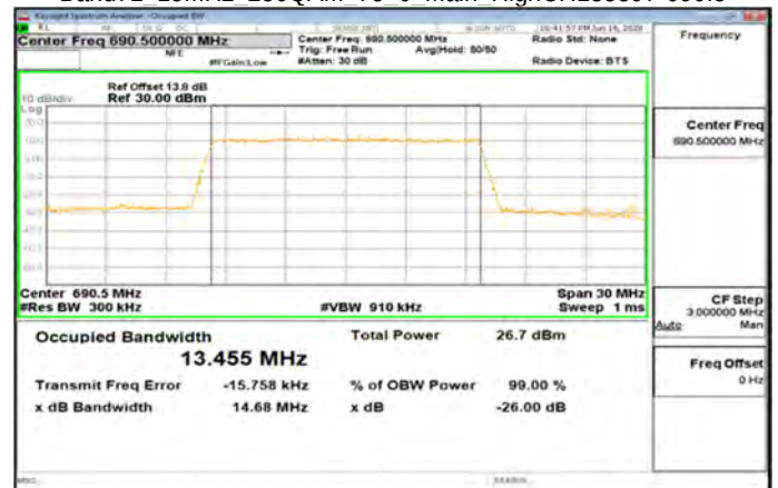
Band71 15MHz 256QAM 75 0 Main HighCH133397-690.5
