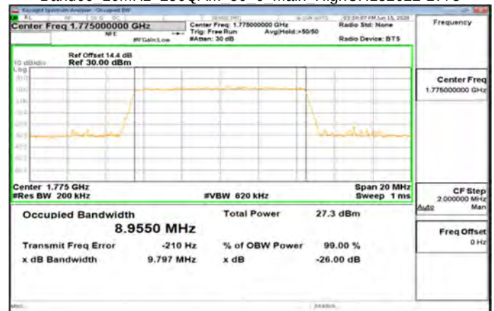
Band66 10MHz 256QAM 50 0 Main HighCH132622-1775
