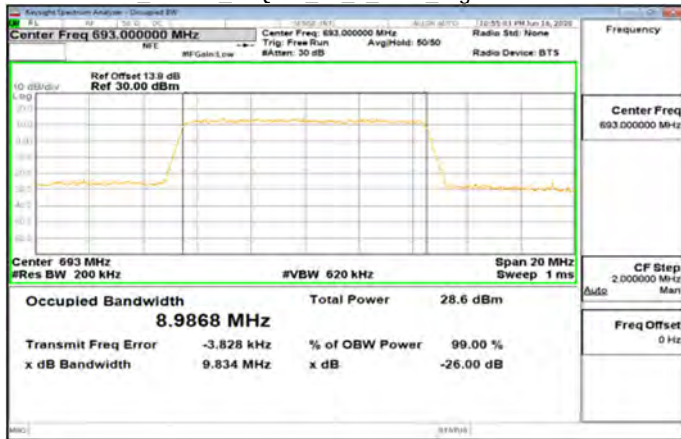
Band71 10MHz 64QAM 50 0 Main HighCH133422-693
