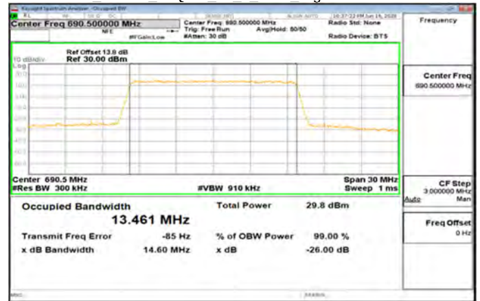
Band71 15MHz 16QAM 75 0 Main HighCH133397-690.5
