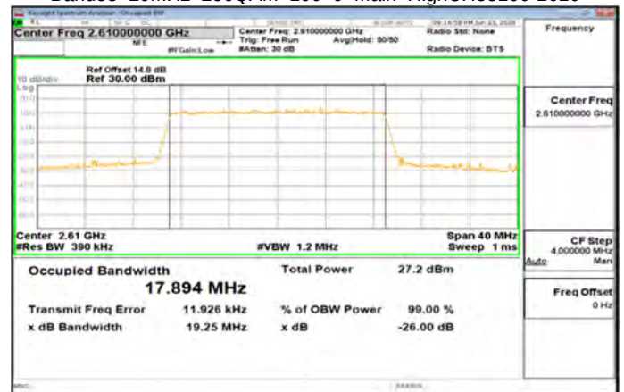
Band38 20MHz 256QAM 100 0 Main HighCH38150-2610
