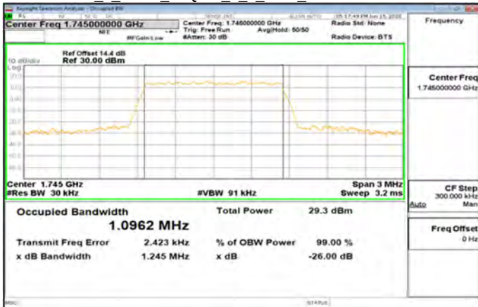
Band66_1_4MHz_64QAM_6_0_Main_MidCH132322-1745
