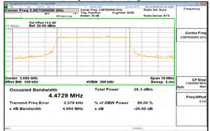
Band41 5MHz 256QAM 25 0 Main HighCH41565-2687.5
