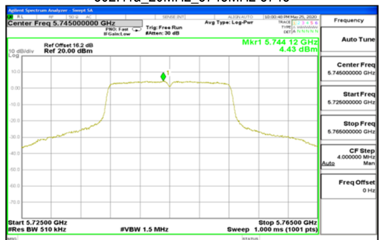
802.11a_20MHz_5745MHz-5745
