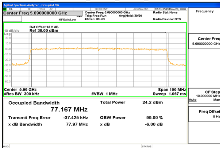
IC_802.11ax_80MHz_Chain1_5690MHz
