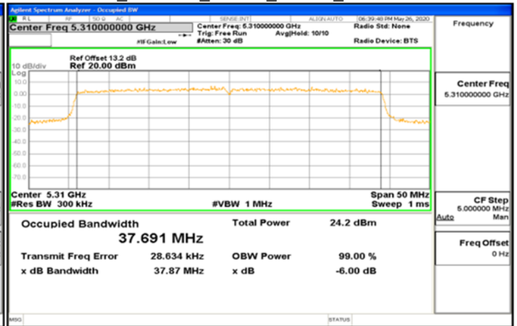
IC_802.11ax_40MHz_Chain0_5310MHz
