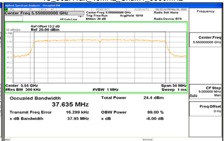
IC_802.11ax_40MHz_Chain1_5550MHz
