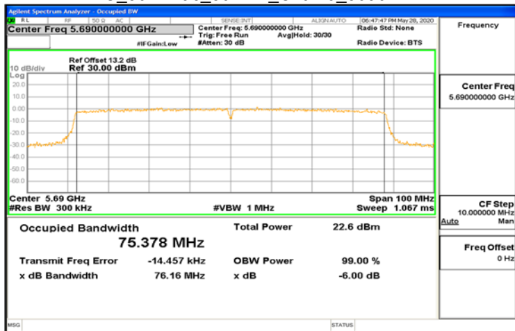
IC_802.11ac_80MHz_Chain0_5690MHz
