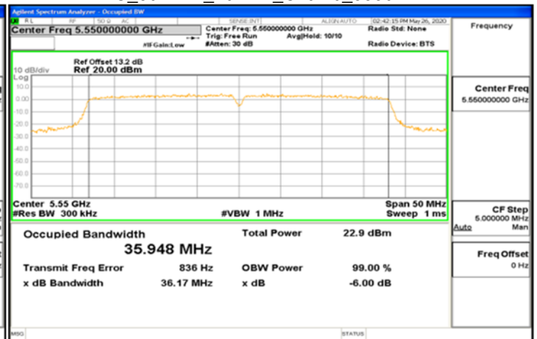
IC_802.11n_40MHz_Chain0_5550MHz
