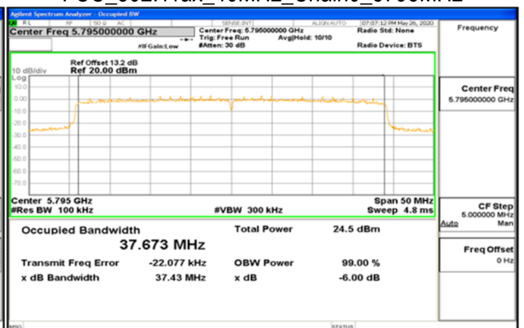
FCC_802.11ax_40MHz_Chain0_5795MHz
