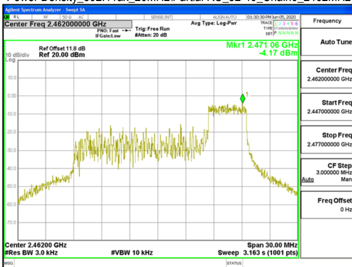
Power Density 802.11ax 20MHz\Partial RU 52-40 Chain0 2462MHz
