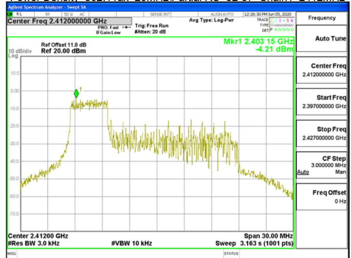
Power Density 802.11ax 20MHz\Partial RU 106-53 Chain0 2412MHz
