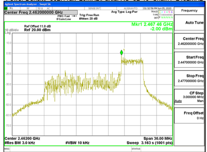
Power Density 802.11ax 20MHz\Partial RU 106-54 Chain0 2462MHz
