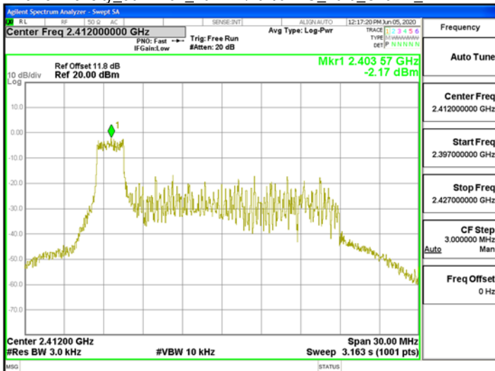
Power Density 802.11ax 20MHz\Partial RU 52-37 Chain0 2412MHz
