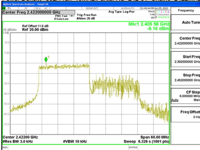
Power Density_802.11ax_40MHz\Partial RU_242-61_Chain1_2422MHz
