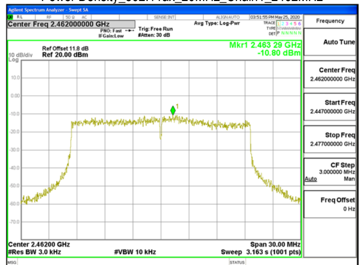
Power Density_802.11ax_20MHz_Chain1_2462MHz
