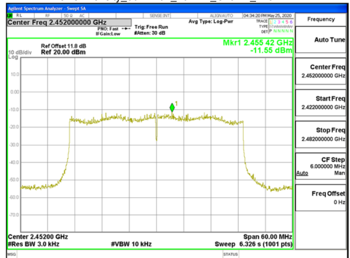
Power Density 802.11ax 40MHz Chain1 2452MHz
