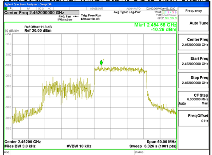
Power Density_802.11ax_40MHz\Partial RU_242-62_Chain1_2452MHz
