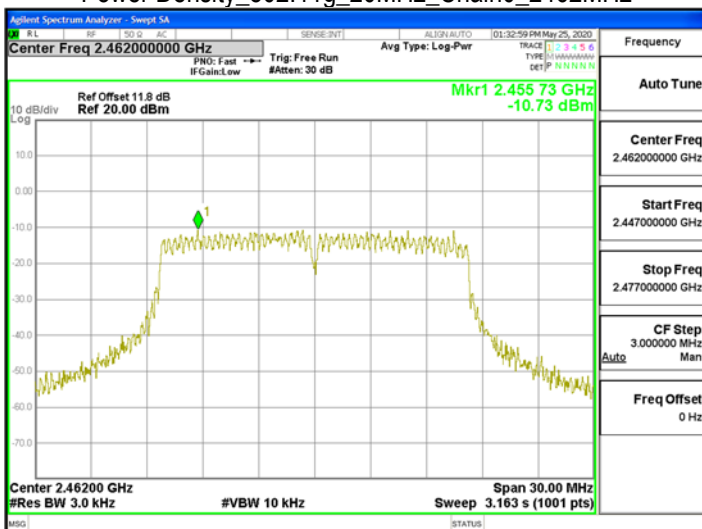
Power Density_802.11g_20MHz_Chain0_2462MHz
