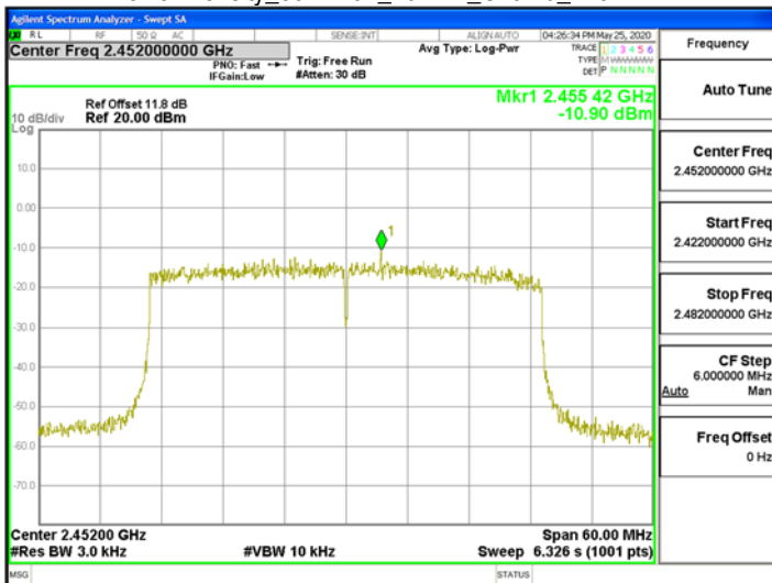
Power Density 802.11ax 40MHz Chain0 2452MHz
