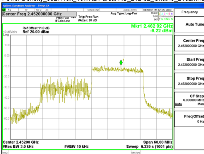
Power Density_802.11ax_40MHz\Partial RU_242-62_Chain0_2452MHz
