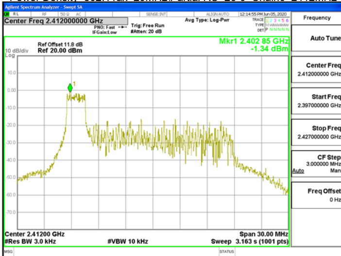
Power Density 802.11ax 20MHz\Partial RU 26-0 Chain1 2412MHz
