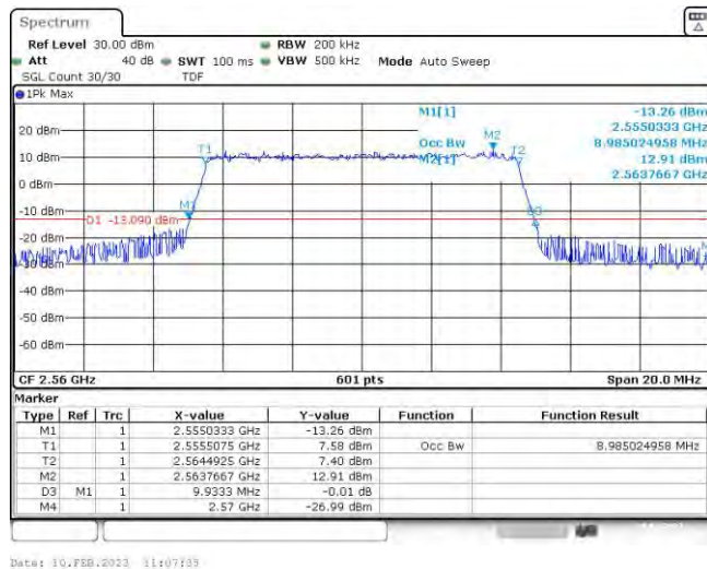
Band41-10MHz-16QAM-40690-50RB#0
