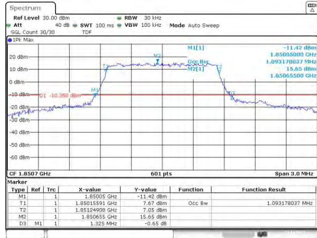
Band2-1.4MHz-QPSK-18607-6RB#0
