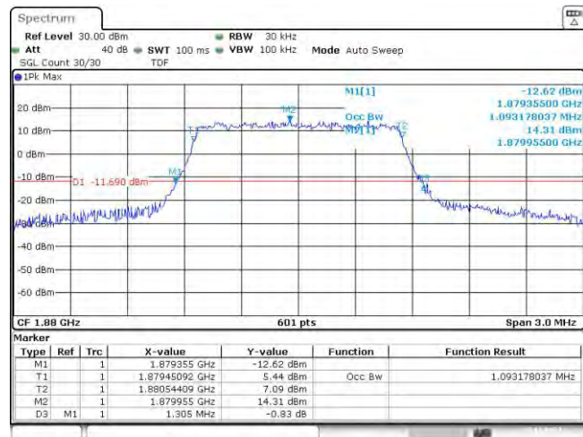
Band2-1.4MHz-QPSK-18900-6RB#0
