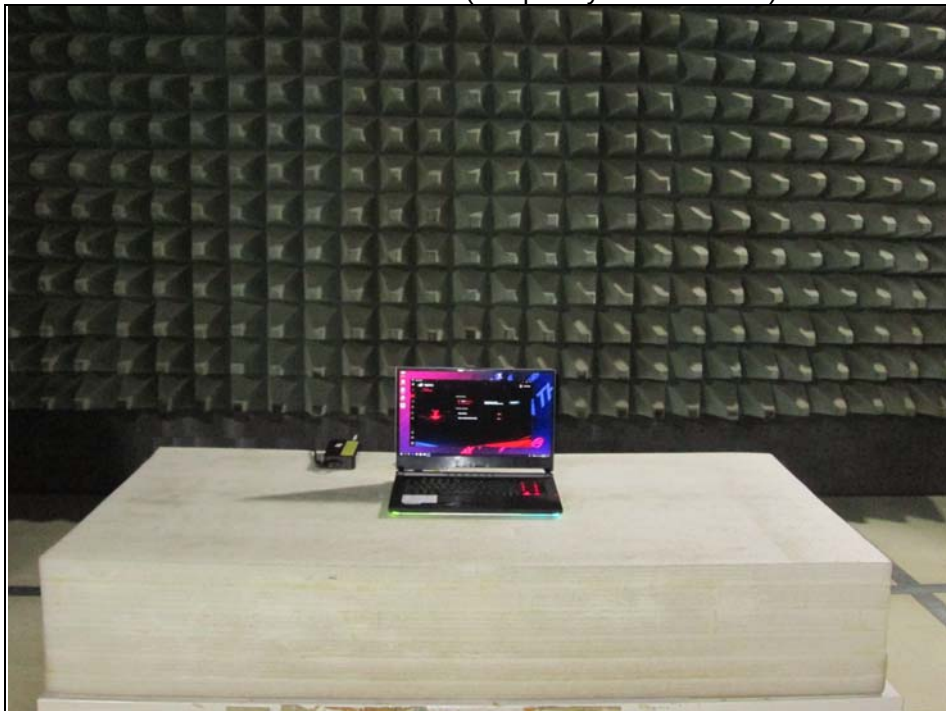
Radiated Emission Test (Frequency below 30MHz)
