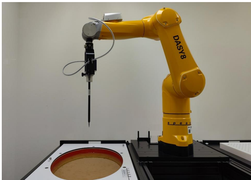
Fig.1 Photograph of the SAR measurement system
