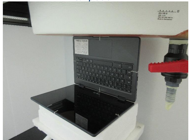
Testing Setup for Body, Front Edge of Laptop at 0 mm, Sample 3 & 4
