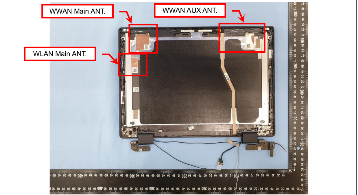
EUT Photo (61) Platform Model Number: CR1104CTA, CR1104FTA, CR1104FG, CR1104CG
