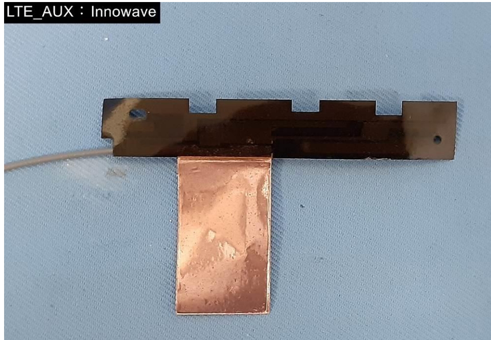
EUT Photo (60) Platform Model Number: CR1204CTA, CR1204FTA, CR1204FG, CR1204CG
