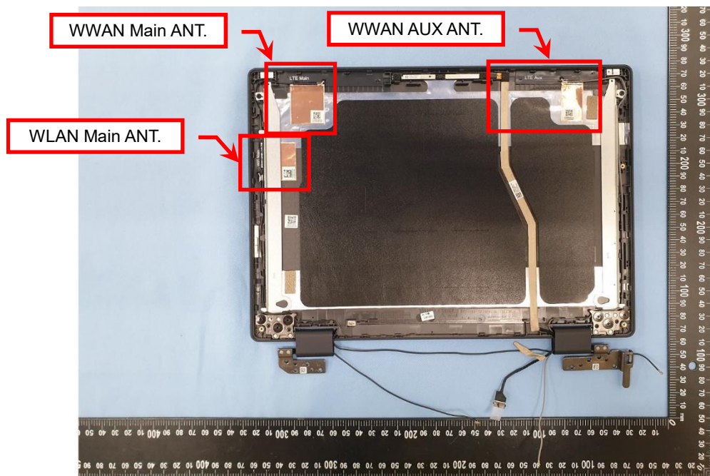
EUT Photo (60) Platform Model Number: CR1204CTA, CR1204FTA, CR1204FG, CR1204CG
