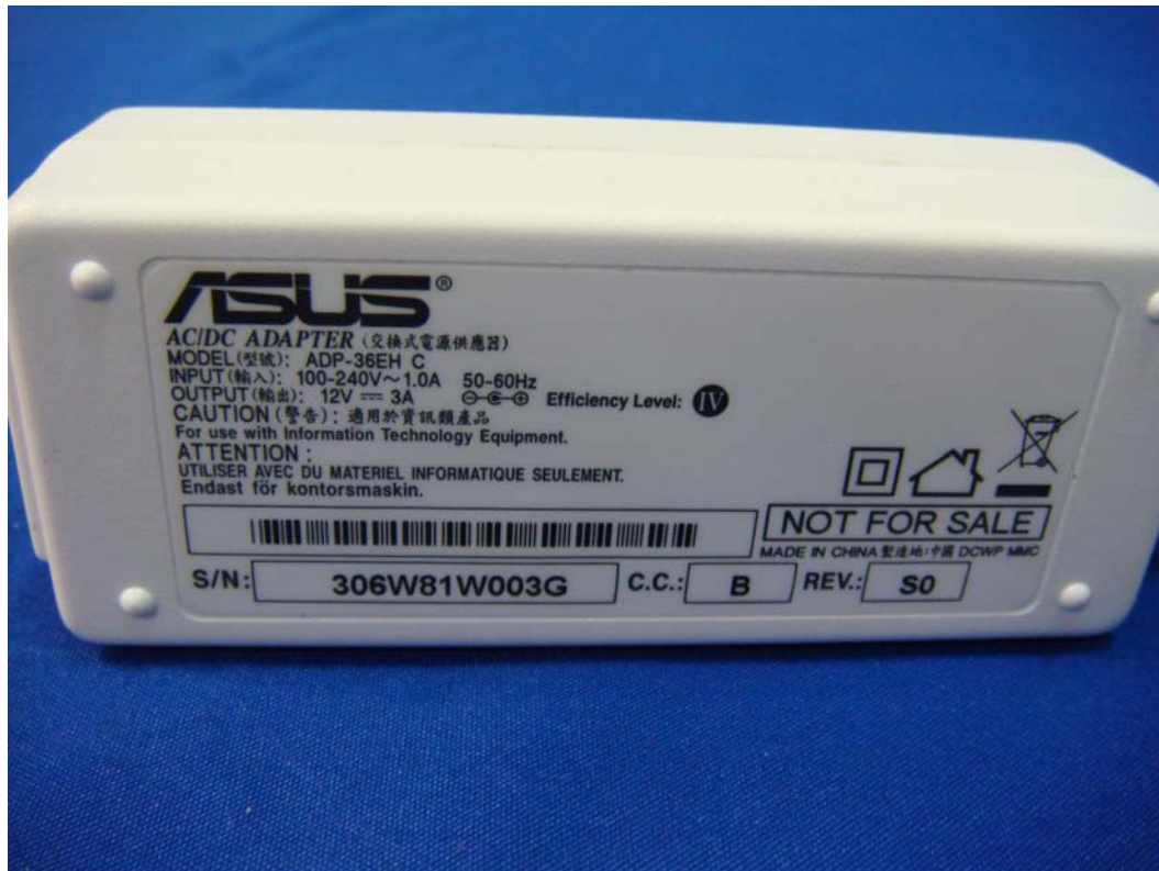
(29) EUT Photo
