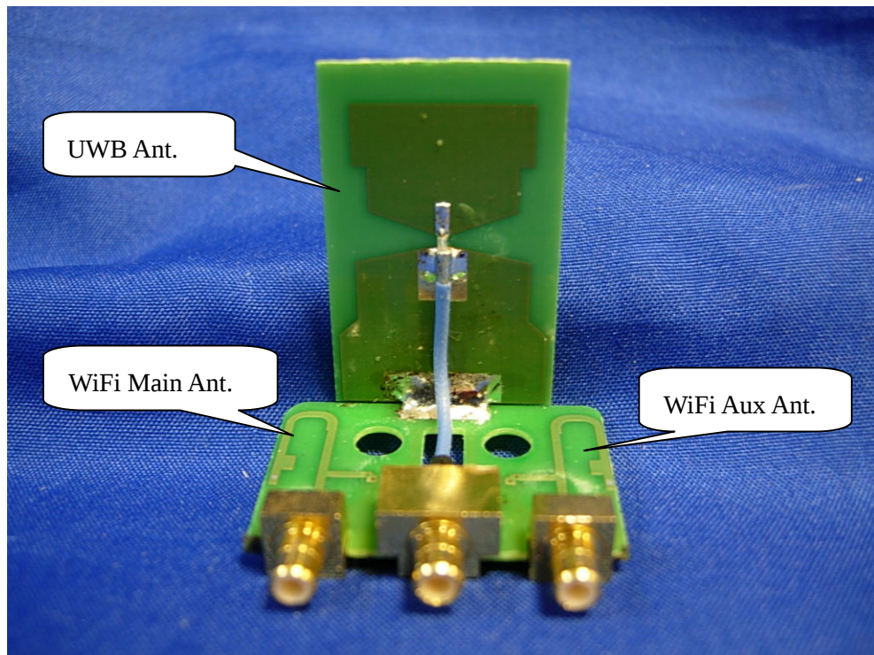
(26) EUT Photo
