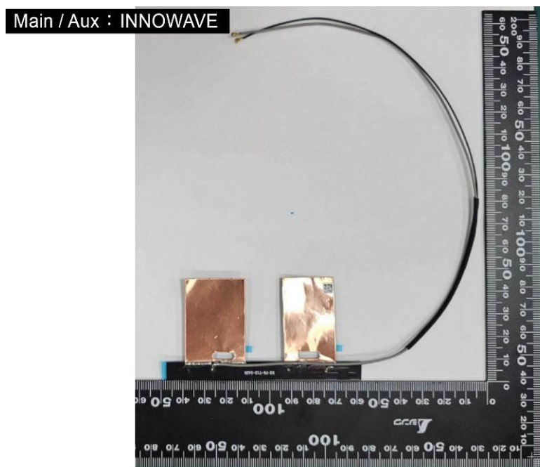
EUT Photo (28)
