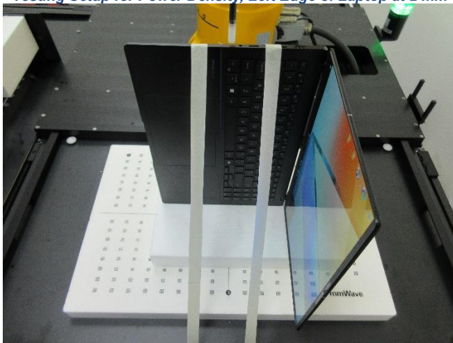
Testing Setup for Power Density, Left Edge of Laptop at 2 mm
