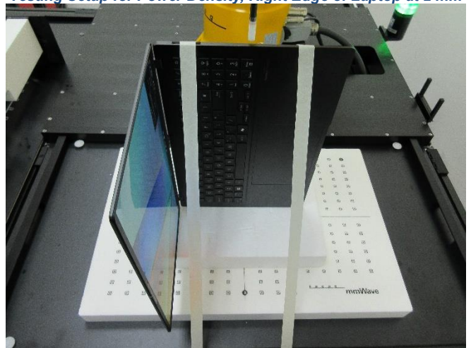
Testing Setup for Power Density, Right Edge of Laptop at 2 mm
