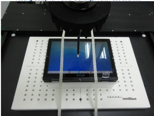
Testing Setup for Power Density, Front Face at 2 mm
