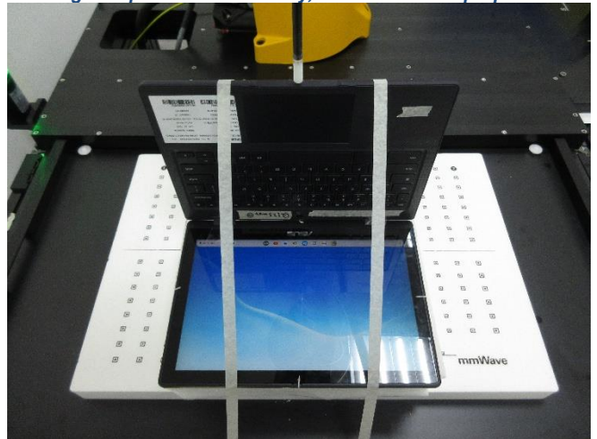
Testing Setup for Power Density, Front Side of Laptop at 2 mm
