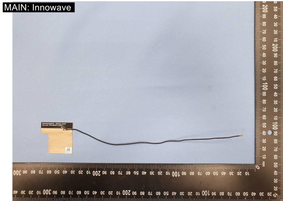
EUT Photo (26)
