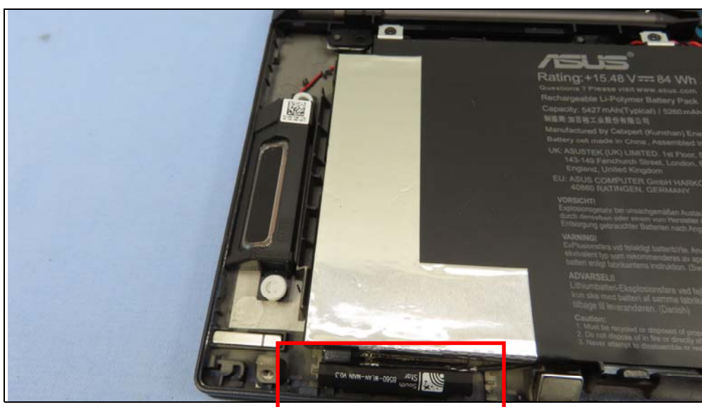
Aux Antenna
