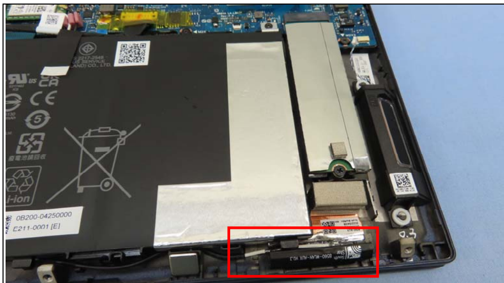
Main Antenna
