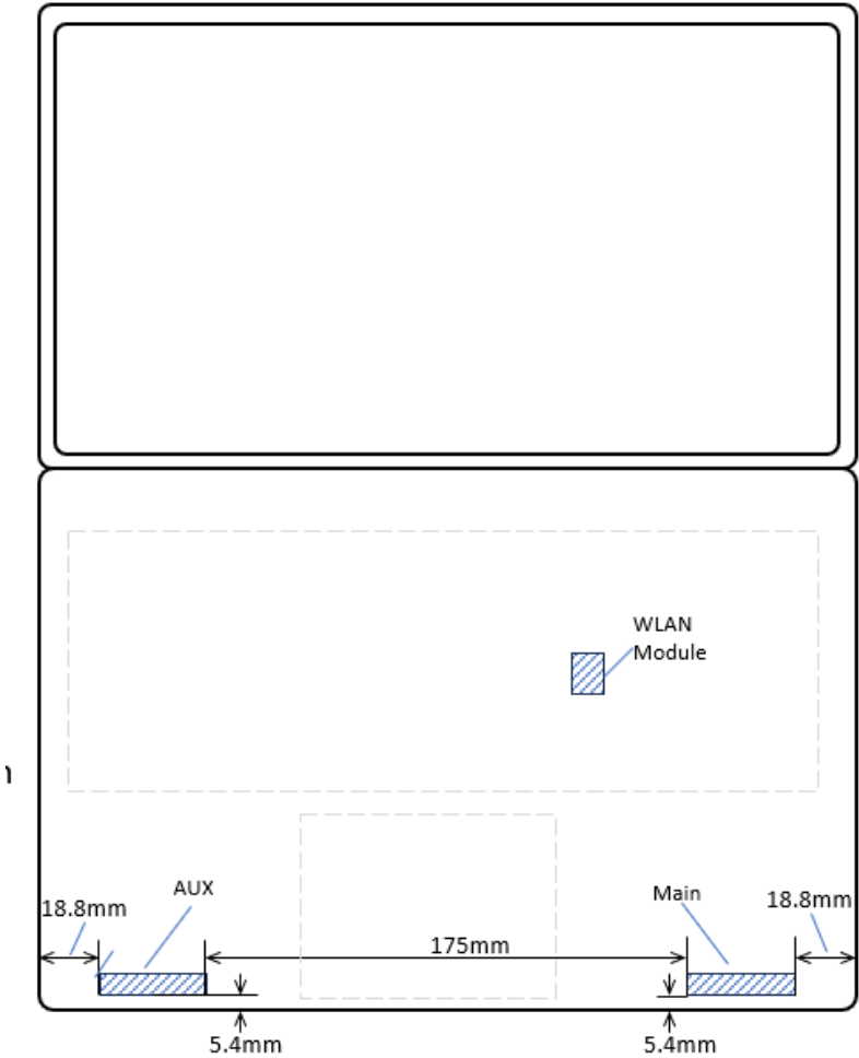
Top View
