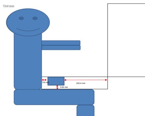
Photograph 7. Antenna position of EUT
