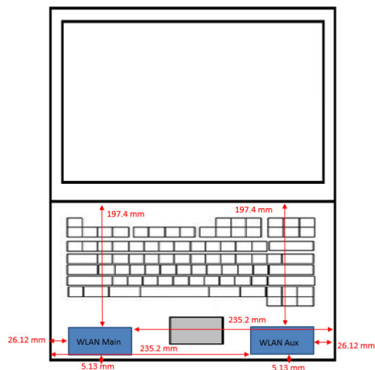
Photograph 19. Antenna position of EUT
