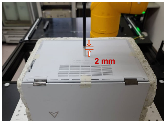
Photograph 13. PD, Bottom Surface, 2mm
