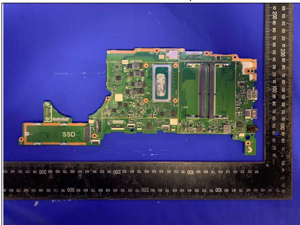
Mother Board - Top
