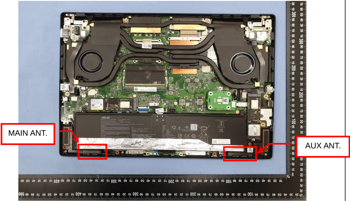
EUT Photo (1)
