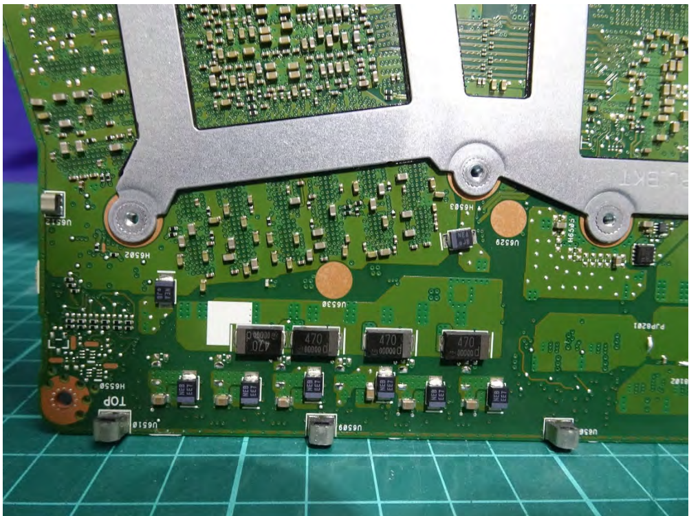
(55) EUT Photo
