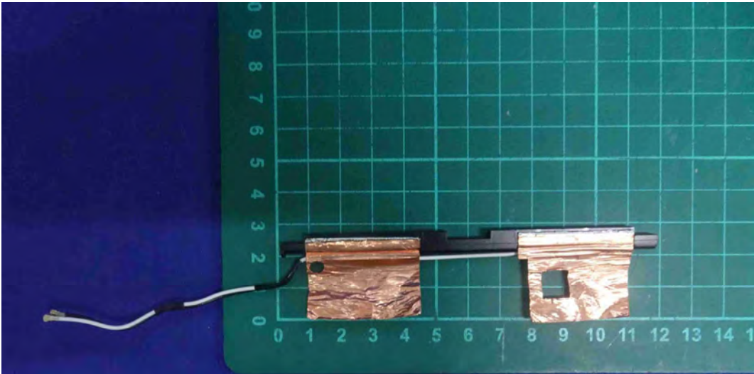
INPAQ Main Antenna Part No. 1415-08EH0A9 WA-F-LBLB-04-07
