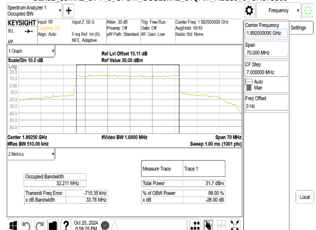
Band2_35MHz_DFT_s_OFDM_SCS15kHz_64QAM_RB180_0_CH378500
