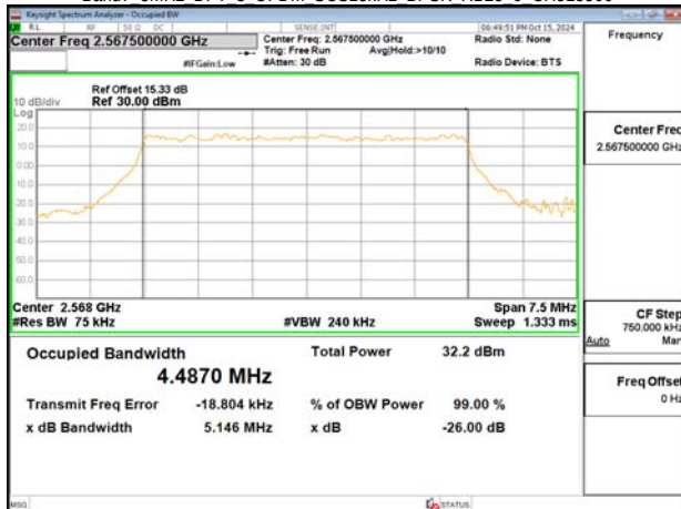
Band7 5MHz DFT s OFDM SCS15kHz BPSK RB25 0 CH513500
