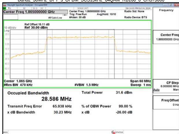
Band2 30MHz DFT s OFDM SCS15kHz 64QAM RB160 0 CH376000
