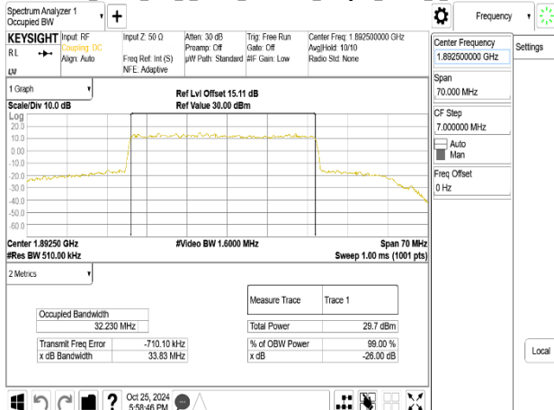
Band2 35MHz DFT_s OFDM_SCS15kHz_256QAM_RB180_0 CH378500
