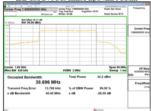
Band2 40MHz DFT s OFDM SCS15kHz 16QAM RB216 0 CH378000
