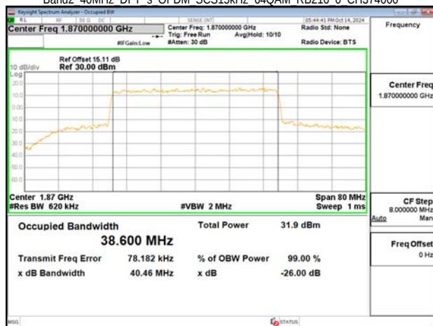
Band2 40MHz DFT s OFDM SCS15kHz 64QAM RB216 0 CH376000
