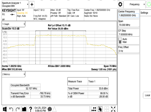
Band2_35MHz_DFT_s_OFDM_SCS15kHz_BPSK_RB180_0_CH378500
