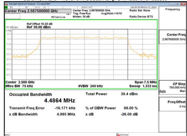
Band7 5MHz DFT s OFDM SCS15kHz QPSK RB25 0 CH513500
