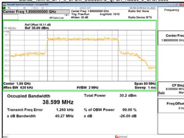
Band2 40MHz DFT s OFDM SCS15kHz QPSK RB216 0 CH378000
