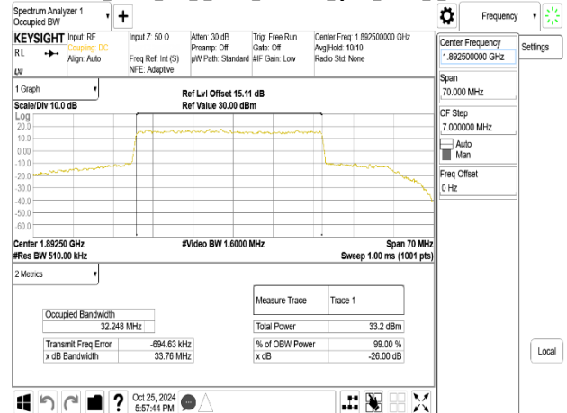
Band2_35MHz_DFT_s_OFDM_SCS15kHz_QPSK_RB180_0_CH378500
