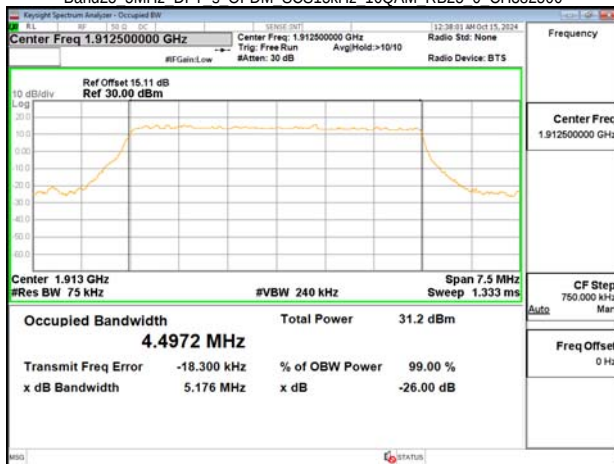
Band25 5MHz DFT s OFDM SCS15kHz 16QAM RB25 0 CH382500
