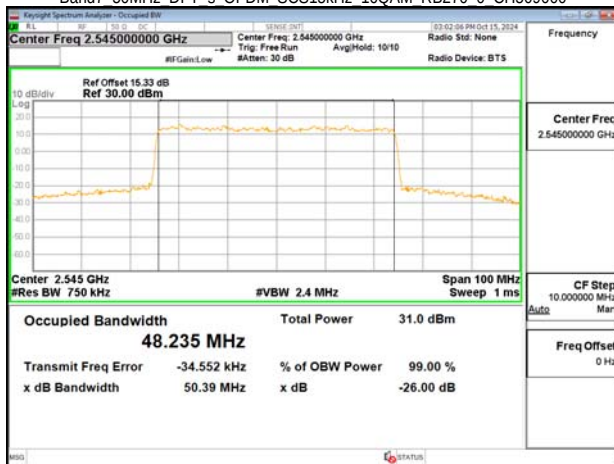
Band7 50MHz DFT s OFDM SCS15kHz 16QAM RB270 0 CH509000
