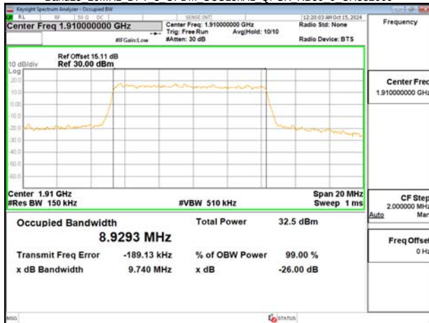
Band25 10MHz DFT s OFDM SCS15kHz QPSK RB50 0 CH382000
