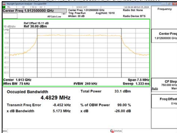
Band25 5MHz DFT s OFDM SCS15kHz BPSK RB25 0 CH382500
