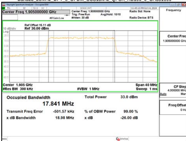
Band25 20MHz DFT s OFDM SCS15kHz QPSK RB100 0 CH381000
