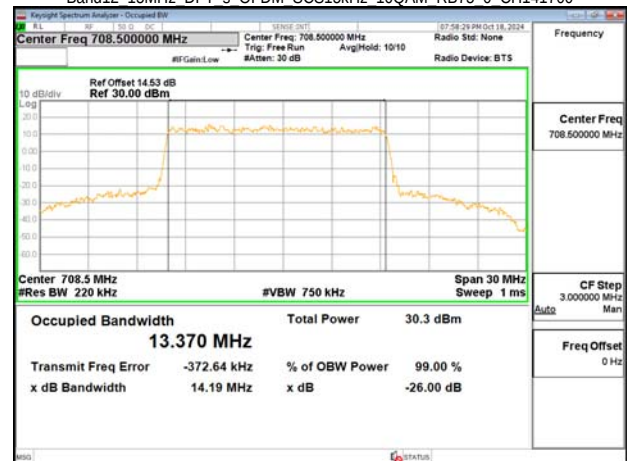
Band12 15MHz DFT s OFDM SCS15kHz 16QAM RB75 0 CH141700
