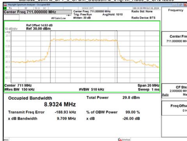
Band12 10MHz DFT s OFDM SCS15kHz 64QAM RB50 0 CH142200
