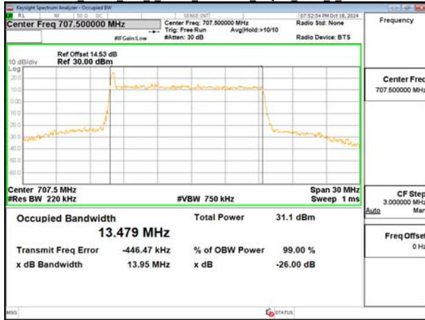
Band12 15MHz DFT s OFDM SCS15kHz 64QAM RB75 0 CH141700
