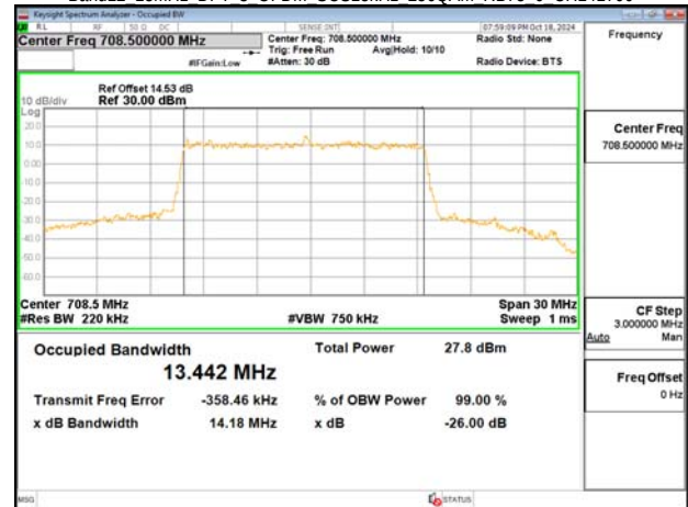
Band12 15MHz DFT s OFDM SCS15kHz 256QAM RB75 0 CH141700
