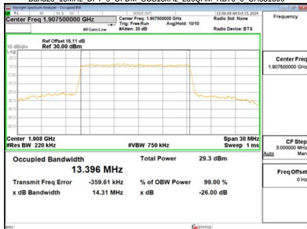
Band25 15MHz DFT s OFDM SCS15kHz 256QAM RB75 0 CH381500
