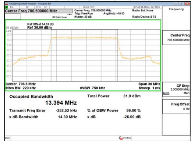
Band12 15MHz DFT s OFDM SCS15kHz BPSK RB75 0 CH141500
