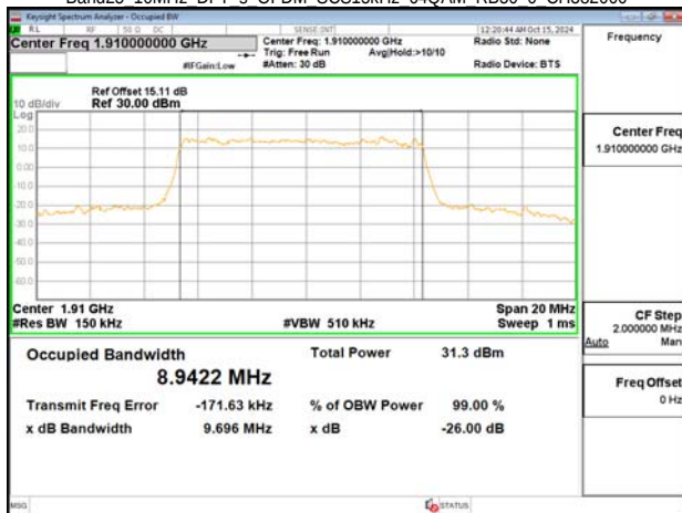
Band25 10MHz DFT s OFDM SCS15kHz 64QAM RB50 0 CH382000
