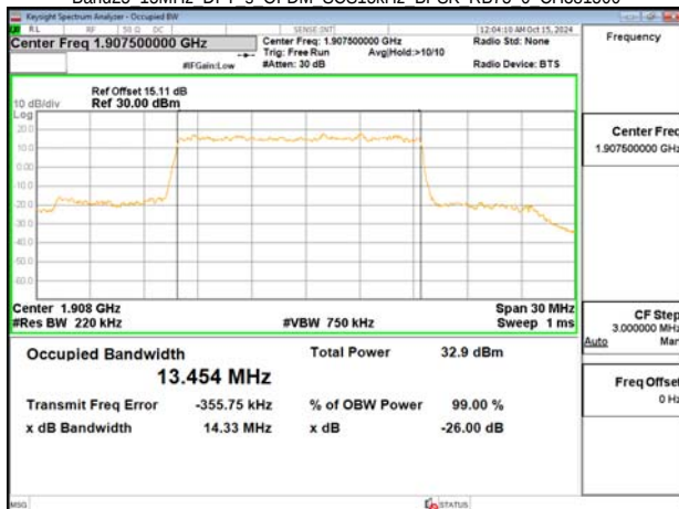
Band25 15MHz DFT s OFDM SCS15kHz BPSK RB75 0 CH381500
