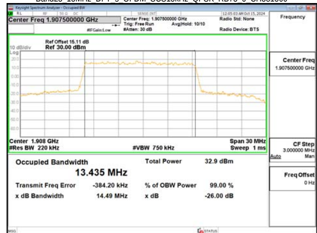
Band25 15MHz DFT s OFDM SCS15kHz QPSK RB75 0 CH381500
