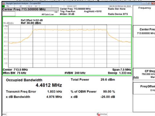
Band12 5MHz DFT s OFDM SCS15kHz 64QAM RB25 0 CH142700
