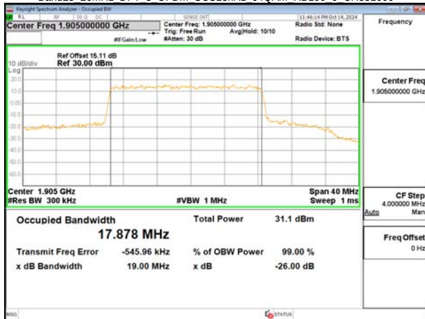
Band25 20MHz DFT s OFDM SCS15kHz 64QAM RB100 0 CH381000
