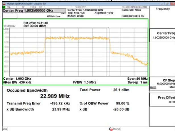
Band25 25MHz DFT s OFDM SCS15kHz 256QAM RB128 0 CH380500
