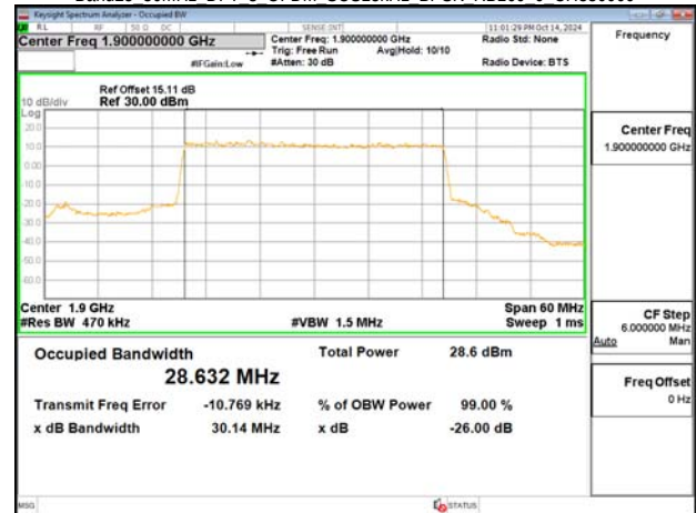
Band25 30MHz DFT s OFDM SCS15kHz BPSK RB160 0 CH380000
