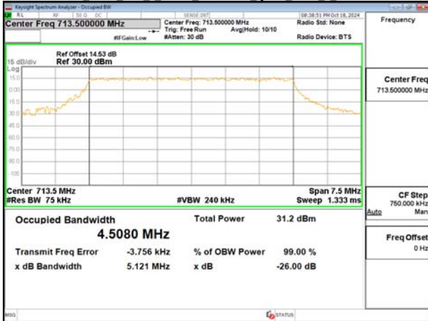
Band12 5MHz DFT s OFDM SCS15kHz QPSK RB25 0 CH142700
