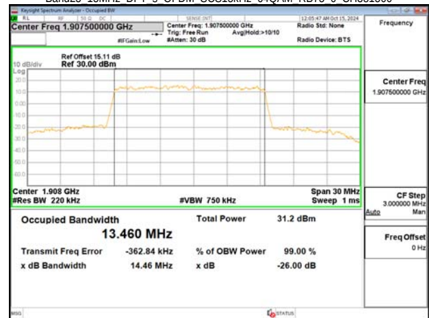
Band25 15MHz DFT s OFDM SCS15kHz 64QAM RB75 0 CH381500
