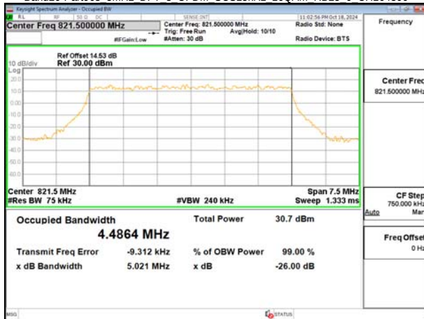
Band26-Part90s 5MHz DFT s OFDM SCS15kHz 16QAM RB25 0 CH164300
