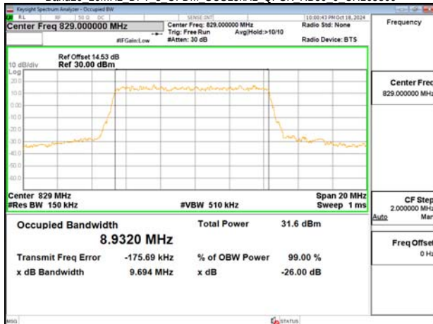
Band26 10MHz DFT s OFDM SCS15kHz QPSK RB50 0 CH165800
