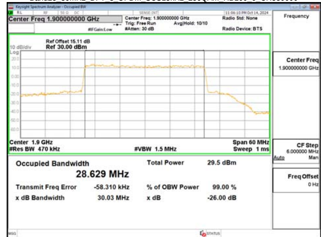
Band25 30MHz DFT s OFDM SCS15kHz 256QAM RB160 0 CH380000
