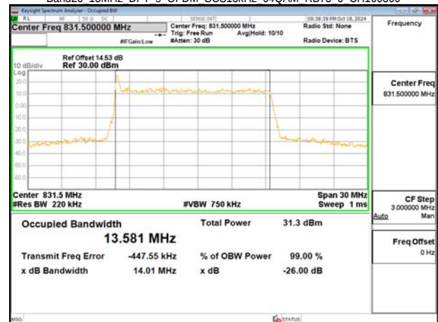
Band26 15MHz DFT s OFDM SCS15kHz 64QAM RB75 0 CH166300
