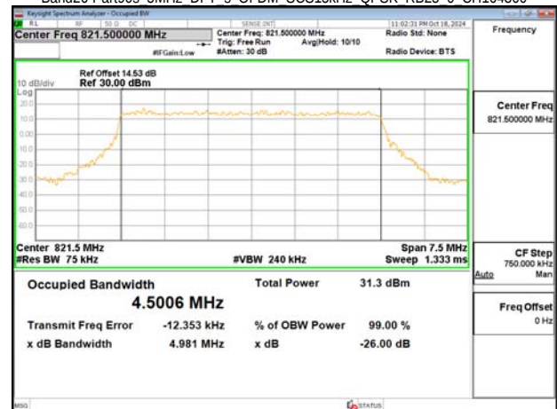
Band26-Part90s 5MHz DFT s OFDM SCS15kHz QPSK RB25 0 CH164300
