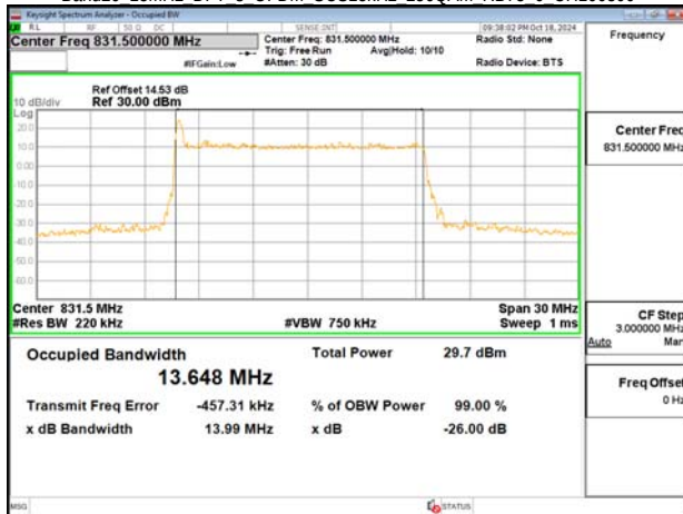
Band26 15MHz DFT s OFDM SCS15kHz 256QAM RB75 0 CH166300
