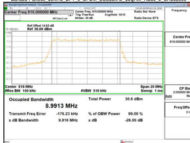
Band26-Part90s 10MHz DFT s OFDM SCS15kHz 16QAM RB50 0 CH163800
