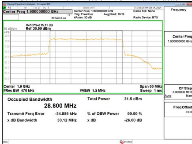
Band25 30MHz DFT s OFDM SCS15kHz 64QAM RB160 0 CH380000
