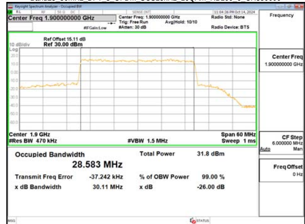
Band25 30MHz DFT s OFDM SCS15kHz 16QAM RB160 0 CH380000
