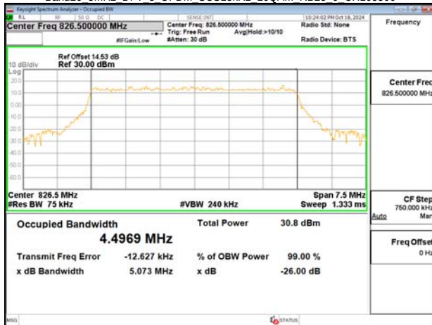
Band26 5MHz DFT s OFDM SCS15kHz 16QAM RB25 0 CH165300
