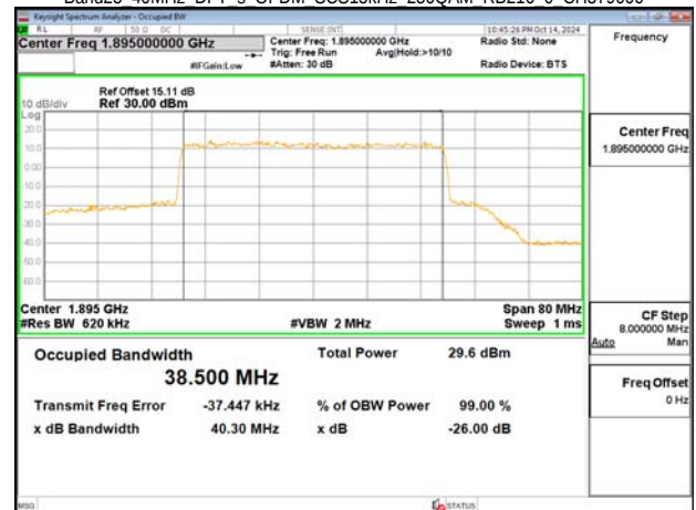
Band25 40MHz DFT s OFDM SCS15kHz 256QAM RB216 0 CH379000
