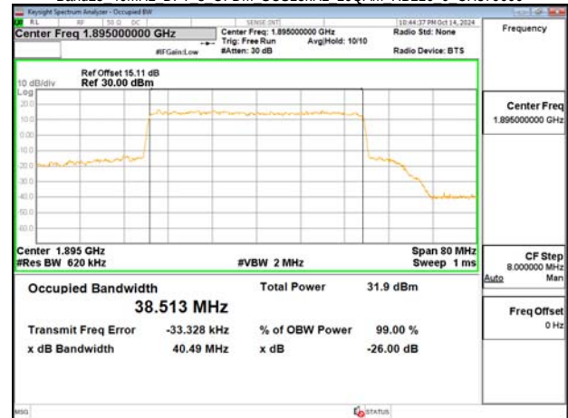
Band25 40MHz DFT s OFDM SCS15kHz 16QAM RB216 0 CH379000
