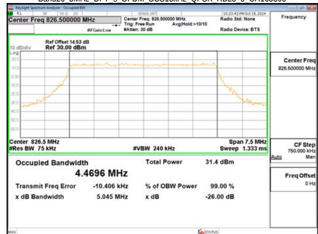
Band26 5MHz DFT s OFDM SCS15kHz QPSK RB25 0 CH165300
