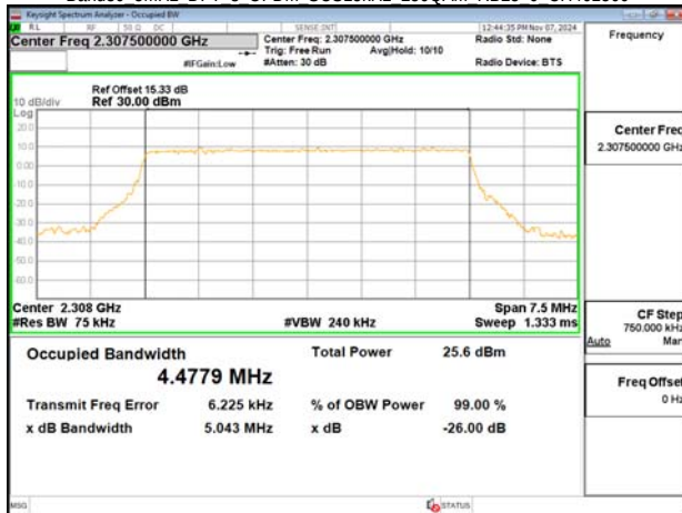
Band30 5MHz DFT s OFDM SCS15kHz 256QAM RB25 0 CH461500
