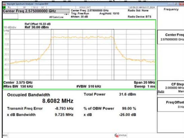
Band38 10MHz DFT s OFDM SCS30kHz QPSK RB24 0 CH519000
