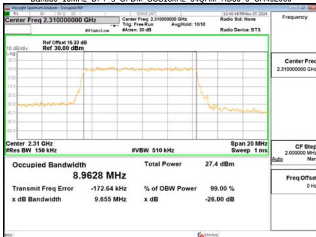
Band30 10MHz DFT s OFDM SCS15kHz 64QAM RB50 0 CH462000
