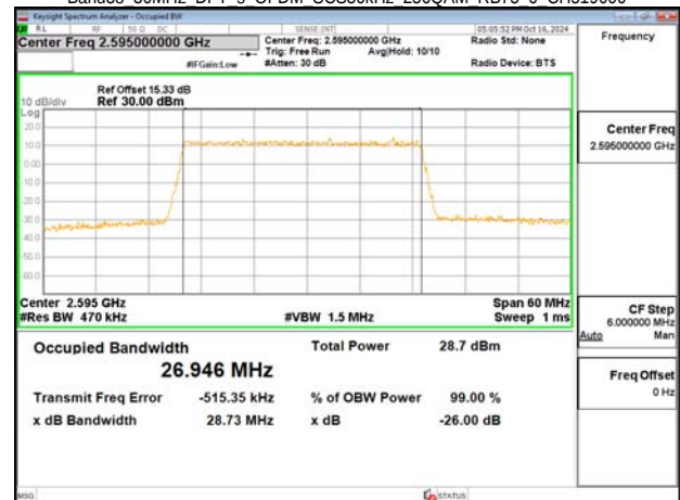
Band38 30MHz DFT s OFDM SCS30kHz 256QAM RB75 0 CH519000
