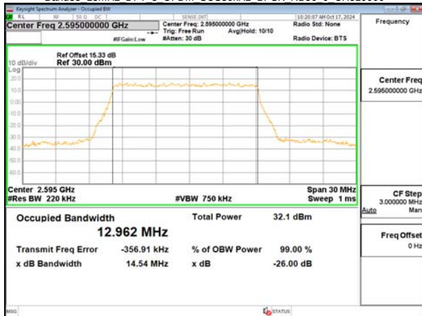
Band38 15MHz DFT s OFDM SCS30kHz BPSK RB36 0 CH519000
