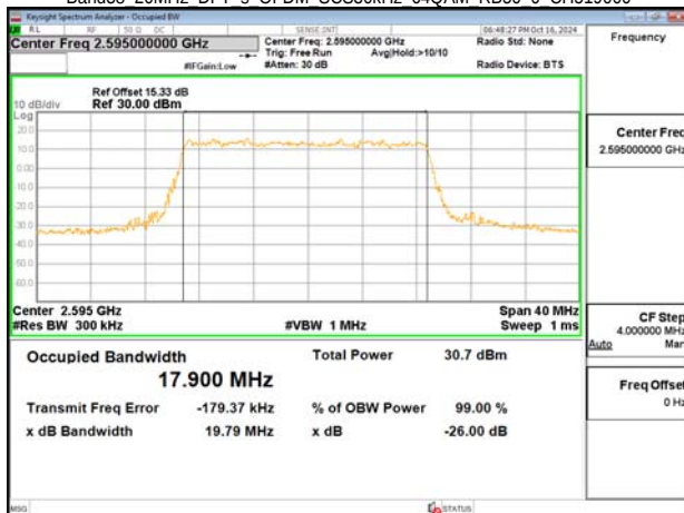
Band38 20MHz DFT s OFDM SCS30kHz 64QAM RB50 0 CH519000
