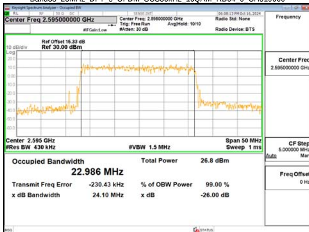
Band38 25MHz DFT s OFDM SCS30kHz 16QAM RB64 0 CH519000
