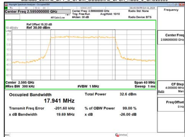
Band38 20MHz DFT s OFDM SCS30kHz BPSK RB50 0 CH519000
