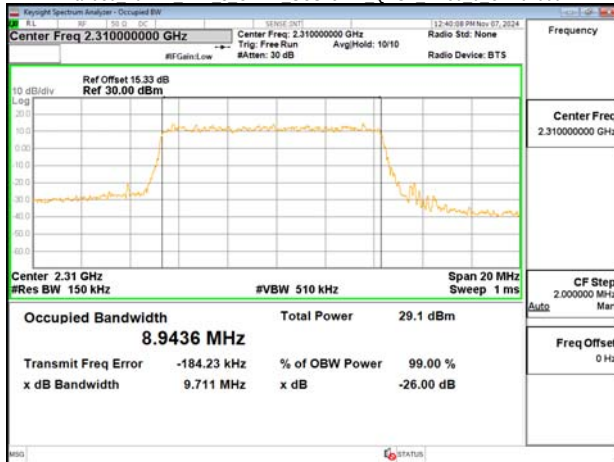
Band30 10MHz DFT s OFDM SCS15kHz 16QAM RB50 0 CH462000
