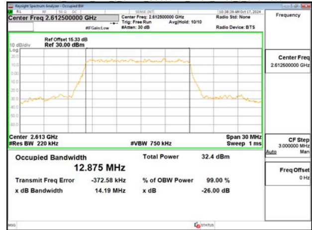
Band38 15MHz DFT s OFDM SCS30kHz QPSK RB36 0 CH515500
