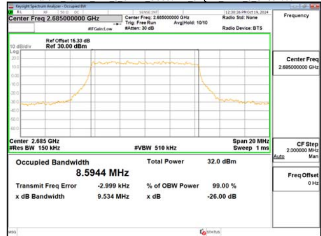
Band41 10MHz DFT s OFDM SCS30kHz 256QAM RB24 0 CH500202
