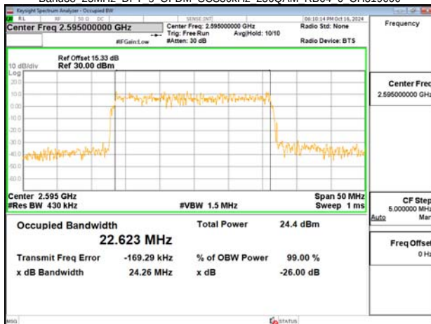
Band38 25MHz DFT s OFDM SCS30kHz 256QAM RB64 0 CH519000
