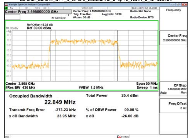
Band38 25MHz DFT s OFDM SCS30kHz 64QAM RB64 0 CH519000
