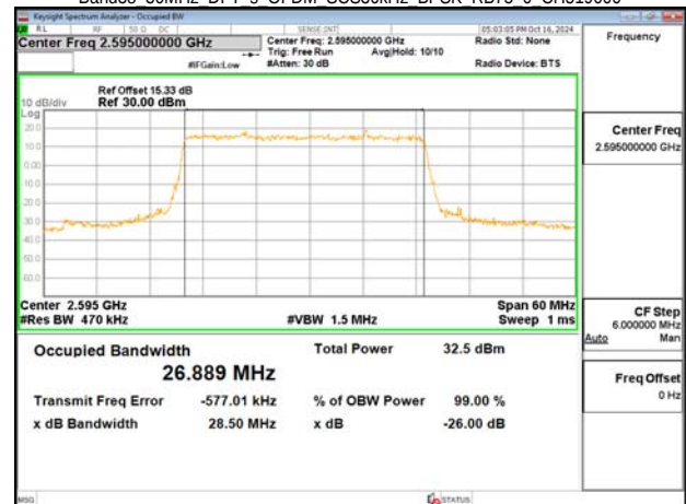
Band38 30MHz DFT s OFDM SCS30kHz BPSK RB75 0 CH519000
