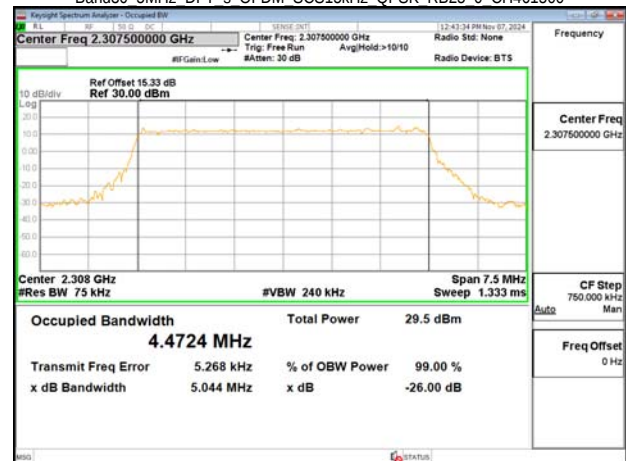
Band30 5MHz DFT s OFDM SCS15kHz QPSK RB25 0 CH461500
