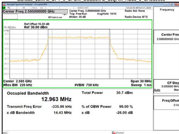
Band38 15MHz DFT s OFDM SCS30kHz 16QAM RB36 0 CH519000
