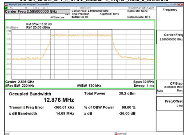
Band38 15MHz DFT s OFDM SCS30kHz 64QAM RB36 0 CH519000
