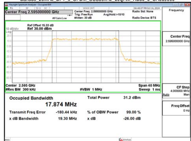
Band38 20MHz DFT s OFDM SCS30kHz 16QAM RB50 0 CH519000
