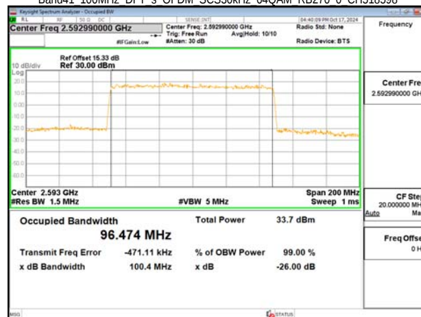
Band41 100MHz DFT s OFDM SCS30kHz 64QAM RB270 0 CH518598
