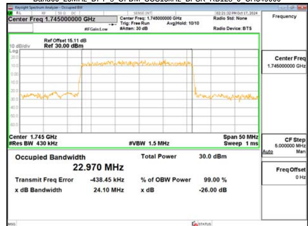
Band66 25MHz DFT s OFDM SCS15kHz BPSK RB128 0 CH349000
