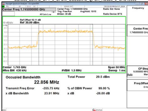
Band66 25MHz DFT s OFDM SCS15kHz QPSK RB128 0 CH349000
