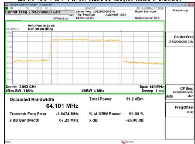
Band41 70MHz DFT s OFDM SCS30kHz 256QAM RB180 0 CH518598
