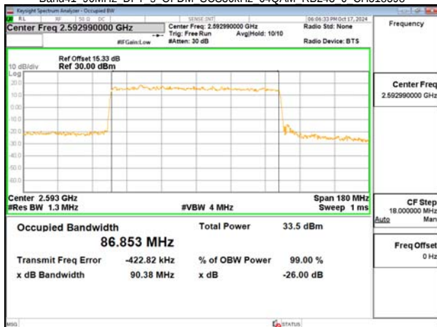
Band41 90MHz DFT s OFDM SCS30kHz 64QAM RB243 0 CH518598
