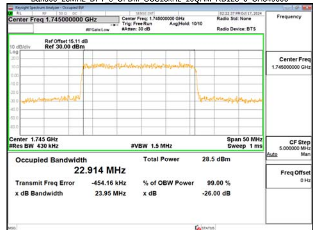
Band66 25MHz DFT s OFDM SCS15kHz 16QAM RB128 0 CH349000
