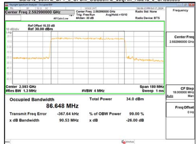
Band41 90MHz DFT s OFDM SCS30kHz 16QAM RB243 0 CH518598
