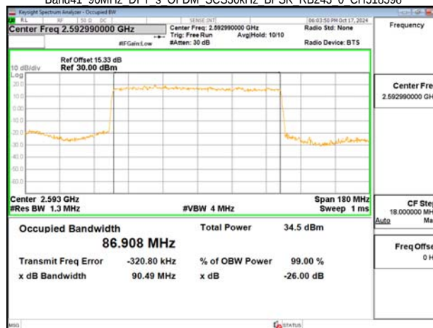
Band41 90MHz DFT s OFDM SCS30kHz BPSK RB243 0 CH518598
