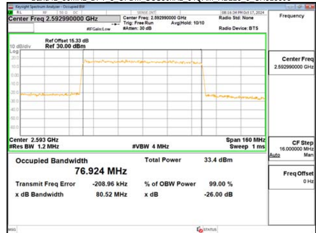
Band41 80MHz DFT s OFDM SCS30kHz 64QAM RB216 0 CH518598
