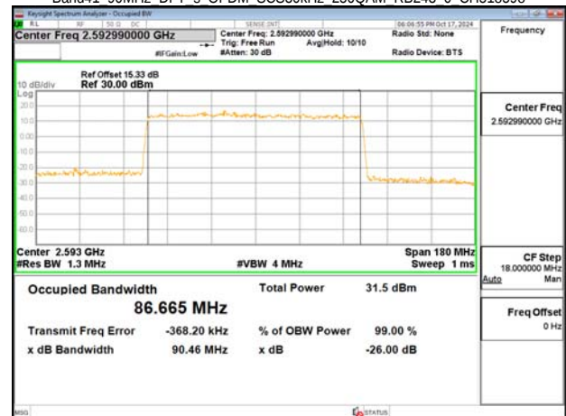
Band41 90MHz DFT s OFDM SCS30kHz 256QAM RB243 0 CH518598
