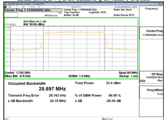
Band66 30MHz DFT s OFDM SCS15kHz QPSK RB160 0 CH349000
