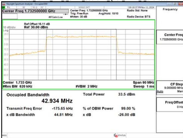
Band66 45MHz DFT s OFDM SCS15kHz QPSK RB242 0 CH349000
