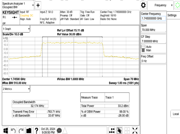
Band66 35MHz DFT_s_OFDM_SCS15kHz_QPSK_RB180_0_CH349000
