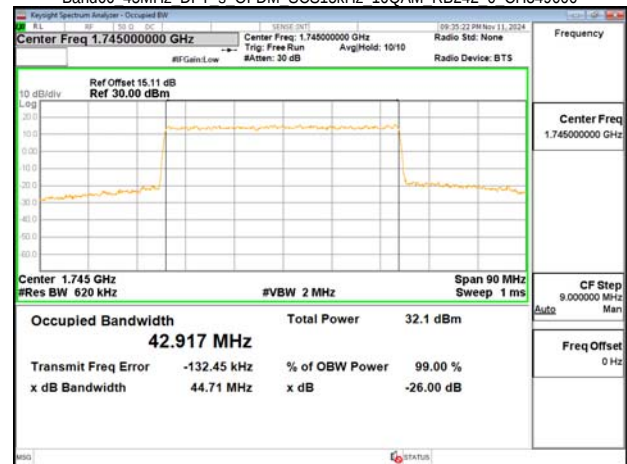
Band66 45MHz DFT s OFDM SCS15kHz 16QAM RB242 0 CH349000
