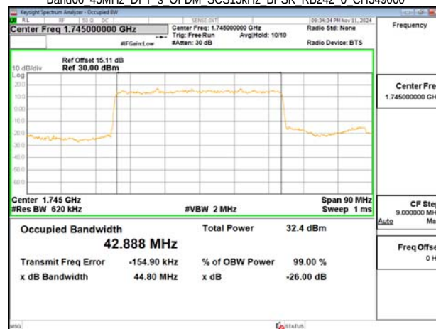
Band66 45MHz DFT s OFDM SCS15kHz BPSK RB242 0 CH349000
