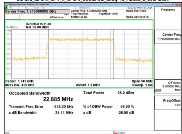
Band66 25MHz DFT s OFDM SCS15kHz 256QAM RB128 0 CH349000
