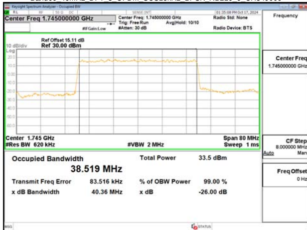
Band66 40MHz DFT s OFDM SCS15kHz BPSK RB216 0 CH349000
