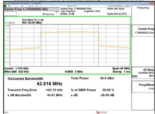
Band66 45MHz DFT s OFDM SCS15kHz 256QAM RB242 0 CH349000
